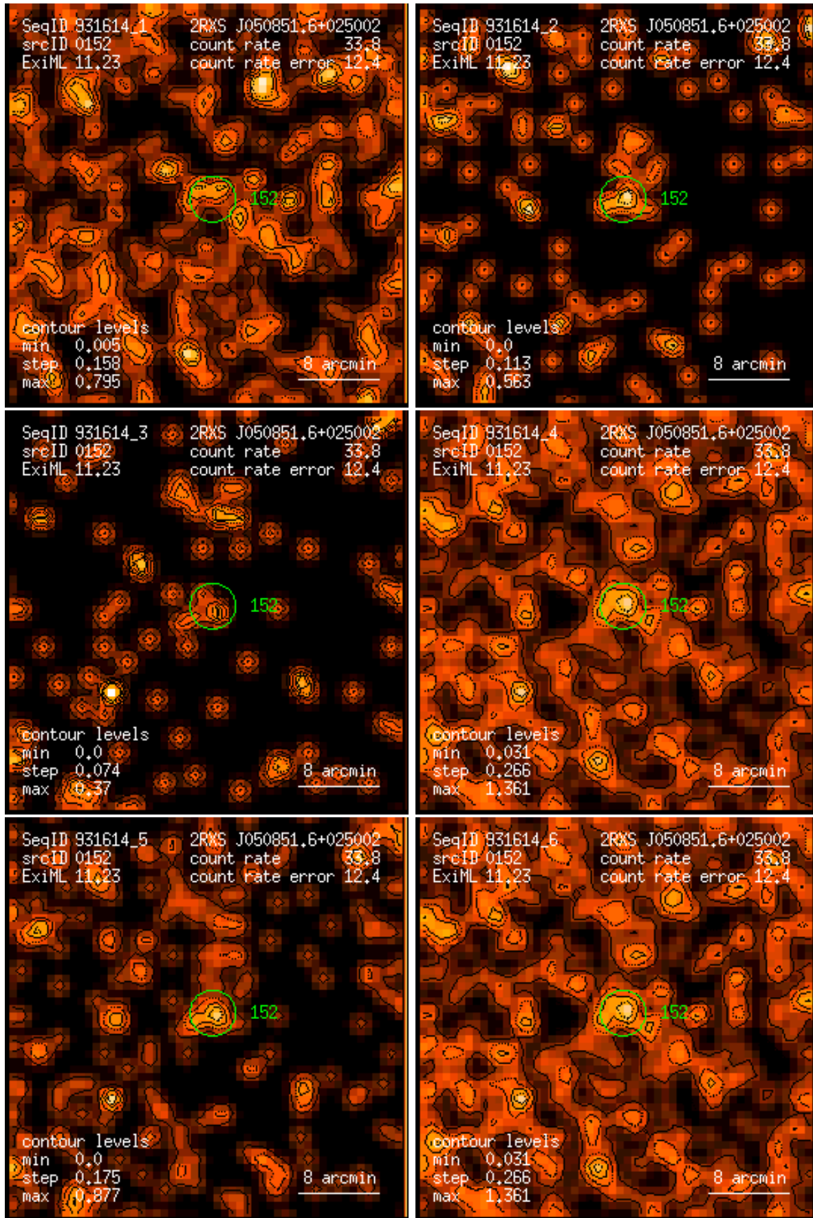
Figure 152: RASS 931614: detection 0152: band rate images, Gaussian filter: (1) PSPC channels 11 – 41, (2) 52 – 90, (3) 91 – 201, (4) 11 – 235, (5) 52 – 201, (6) 11 – 201. Broad band rates in counts/ks. Band rate contour levels in counts/ks/arcmin 2 .
