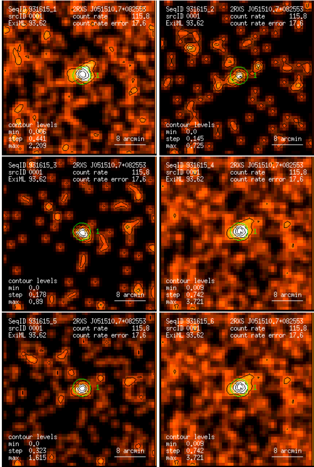
Figure 1: RASS 931615: detection 0001: band rate images, Gaussian filter: (1) PSPC channels 11 – 41, (2) 52 – 90, (3) 91 – 201, (4) 11 – 235, (5) 52 – 201, (6) 11 – 201. Broad band rates in counts/ks. Band rate contour levels in counts/ks/arcmin 2 .
