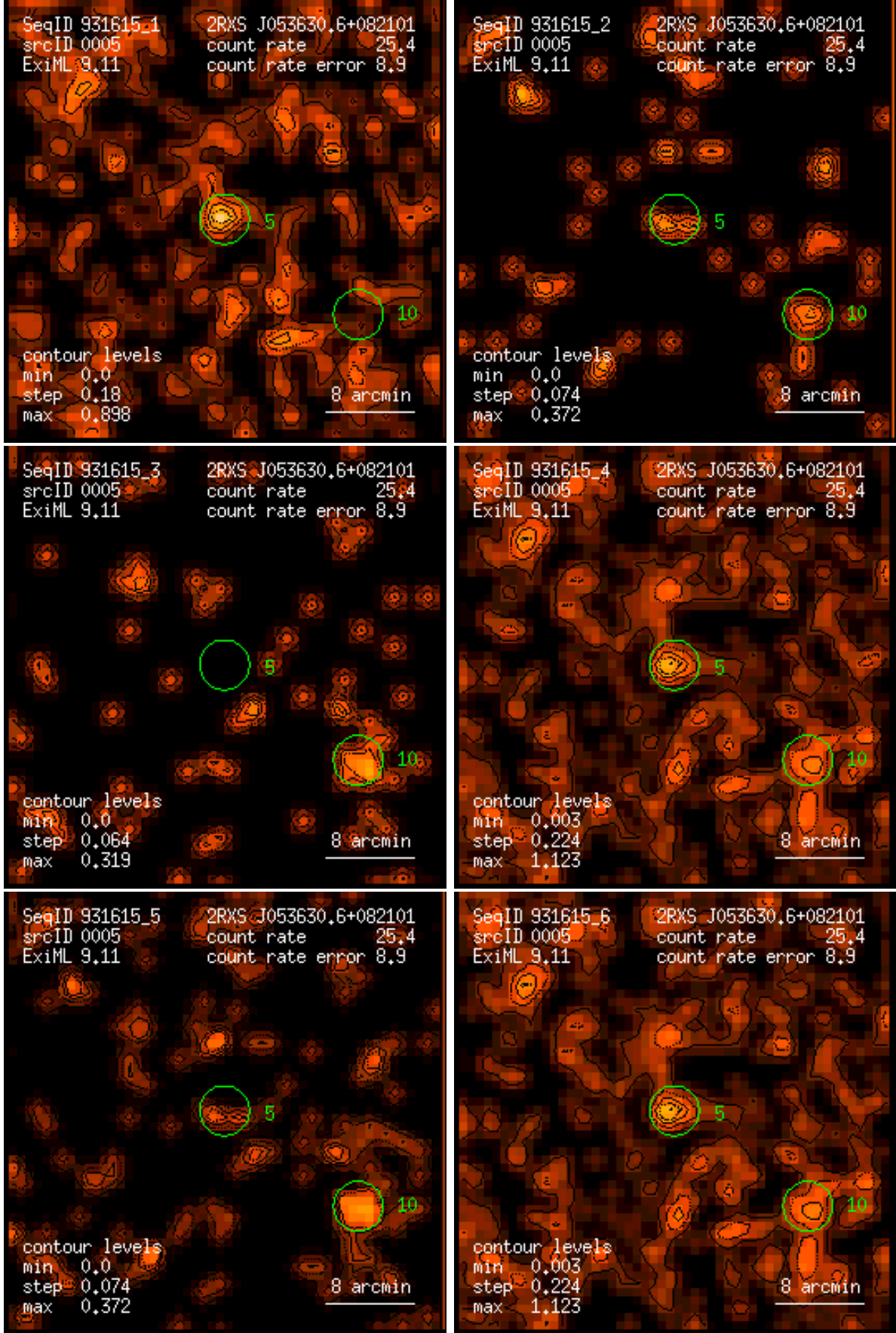
Figure 5: RASS 931615: detection 0005: band rate images, Gaussian filter: (1) PSPC channels 11 – 41, (2) 52 – 90, (3) 91 – 201, (4) 11 – 235, (5) 52 – 201, (6) 11 – 201. Broad band rates in counts/ks. Band rate contour levels in counts/ks/arcmin 2 .
