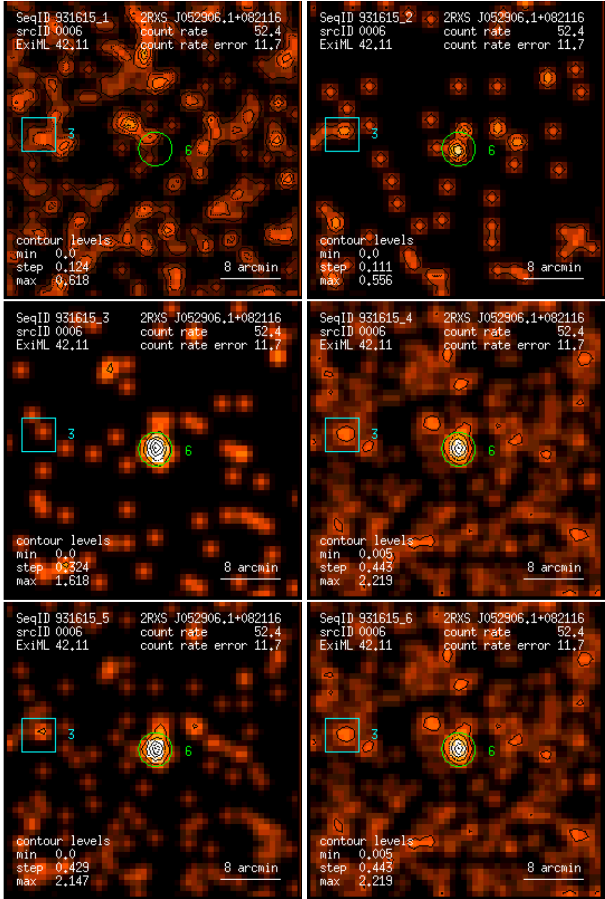
Figure 6: RASS 931615: detection 0006: band rate images, Gaussian filter: (1) PSPC channels 11 – 41, (2) 52 – 90, (3) 91 – 201, (4) 11 – 235, (5) 52 – 201, (6) 11 – 201. Broad band rates in counts/ks. Band rate contour levels in counts/ks/arcmin 2 .
