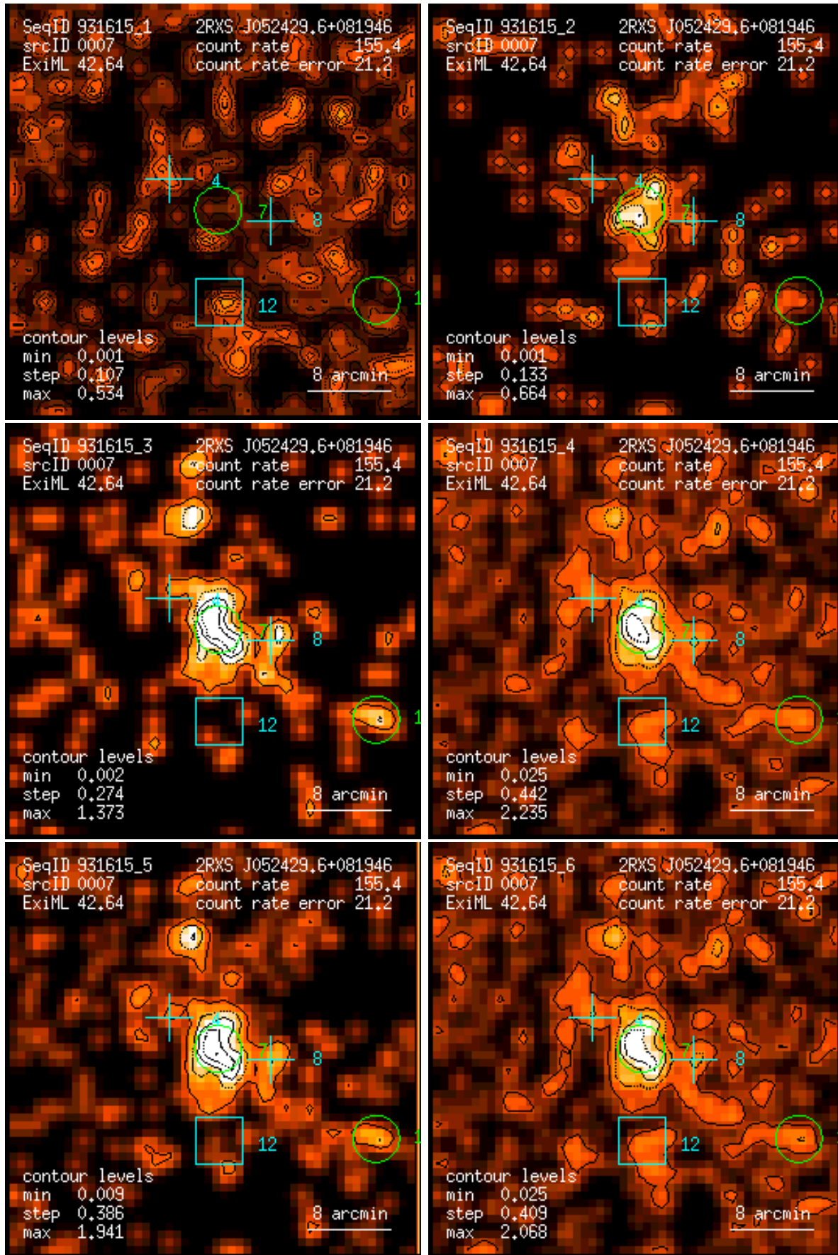
Figure 7: RASS 931615: detection 0007: band rate images, Gaussian filter: (1) PSPC channels 11 – 41, (2) 52 – 90, (3) 91 – 201, (4) 11 – 235, (5) 52 – 201, (6) 11 – 201. Broad band rates in counts/ks. Band rate contour levels in counts/ks/arcmin 2 .
