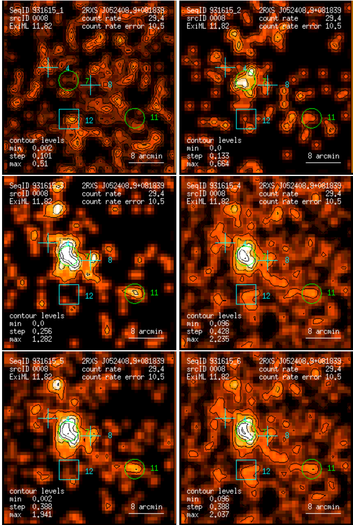
Figure 8: RASS 931615: detection 0008: band rate images, Gaussian filter: (1) PSPC channels 11 – 41, (2) 52 – 90, (3) 91 – 201, (4) 11 – 235, (5) 52 – 201, (6) 11 – 201. Broad band rates in counts/ks. Band rate contour levels in counts/ks/arcmin 2 .
