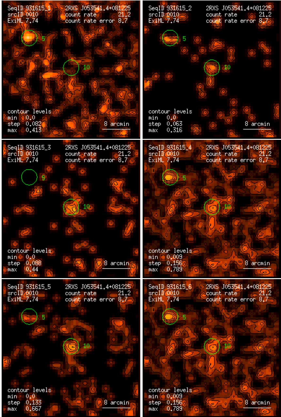
Figure 10: RASS 931615: detection 0010: band rate images, Gaussian filter: (1) PSPC channels 11 – 41, (2) 52 – 90, (3) 91 – 201, (4) 11 – 235, (5) 52 – 201, (6) 11 – 201. Broad band rates in counts/ks. Band rate contour levels in counts/ks/arcmin 2 .
