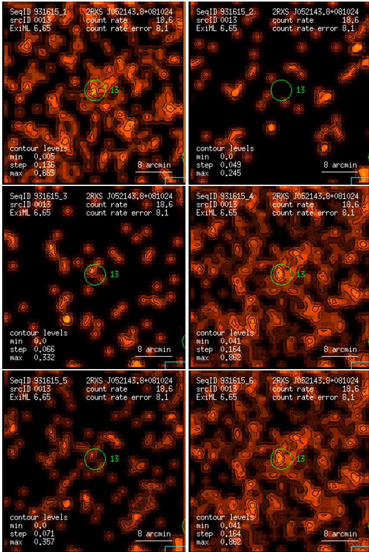
Figure 13: RASS 931615: detection 0013: band rate images, Gaussian filter: (1) PSPC channels 11 – 41, (2) 52 – 90, (3) 91 – 201, (4) 11 – 235, (5) 52 – 201, (6) 11 – 201. Broad band rates in counts/ks. Band rate contour levels in counts/ks/arcmin 2 .
