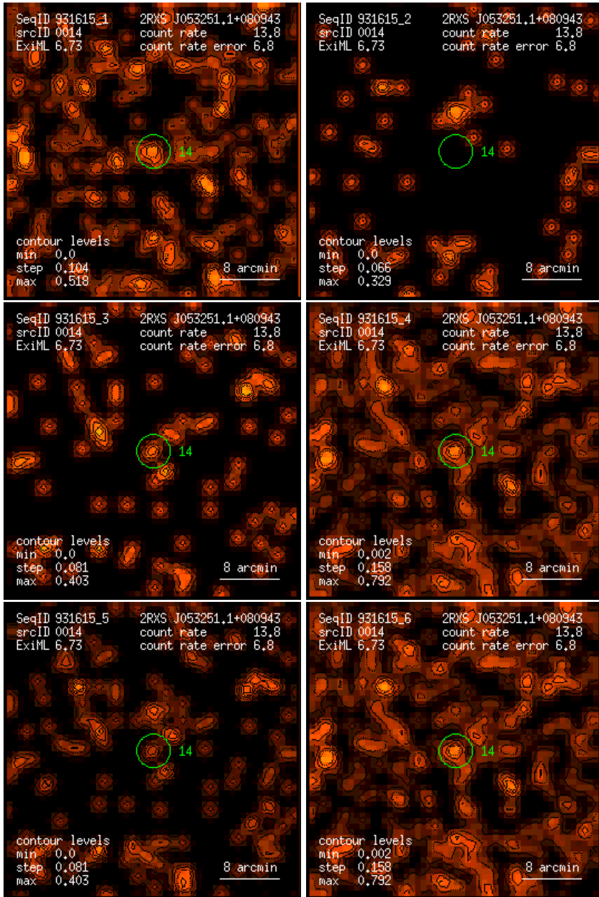
Figure 14: RASS 931615: detection 0014: band rate images, Gaussian filter: (1) PSPC channels 11 – 41, (2) 52 – 90, (3) 91 – 201, (4) 11 – 235, (5) 52 – 201, (6) 11 – 201. Broad band rates in counts/ks. Band rate contour levels in counts/ks/arcmin 2 .
