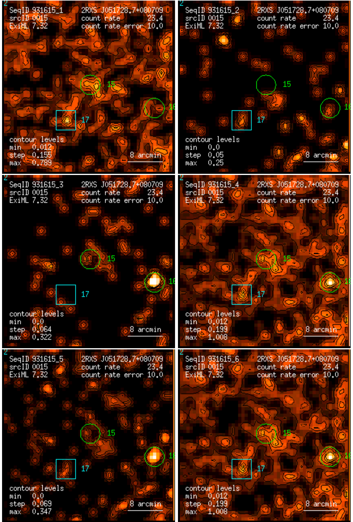
Figure 15: RASS 931615: detection 0015: band rate images, Gaussian filter: (1) PSPC channels 11 – 41, (2) 52 – 90, (3) 91 – 201, (4) 11 – 235, (5) 52 – 201, (6) 11 – 201. Broad band rates in counts/ks. Band rate contour levels in counts/ks/arcmin 2 .
