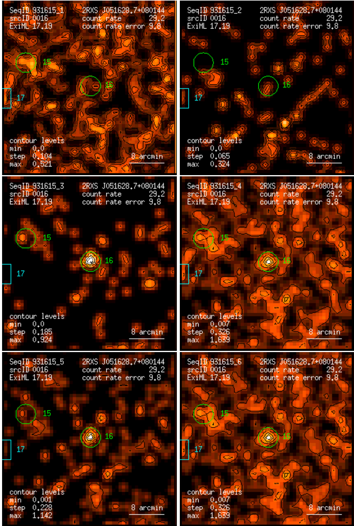
Figure 16: RASS 931615: detection 0016: band rate images, Gaussian filter: (1) PSPC channels 11 – 41, (2) 52 – 90, (3) 91 – 201, (4) 11 – 235, (5) 52 – 201, (6) 11 – 201. Broad band rates in counts/ks. Band rate contour levels in counts/ks/arcmin 2 .
