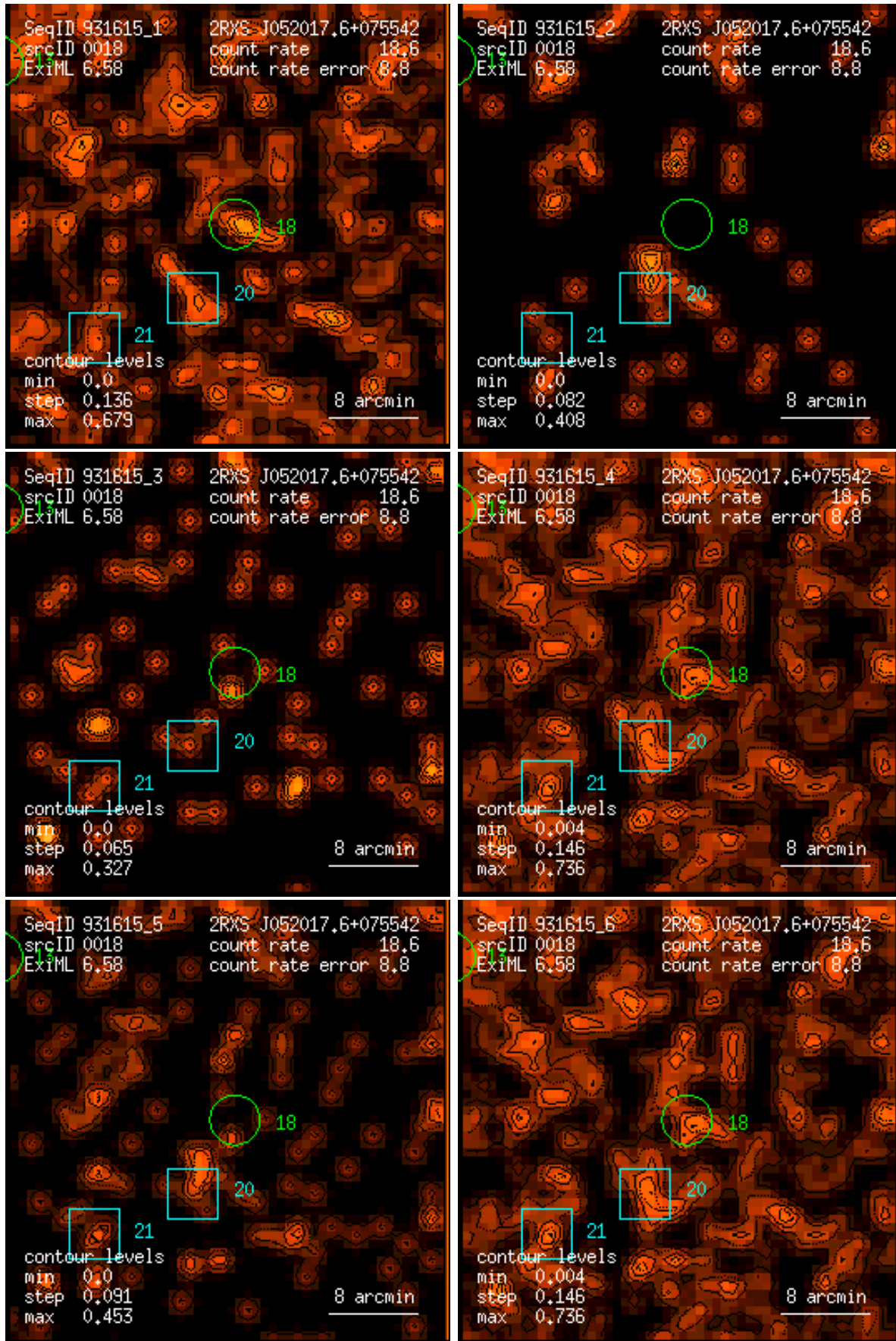
Figure 18: RASS 931615: detection 0018: band rate images, Gaussian filter: (1) PSPC channels 11 – 41, (2) 52 – 90, (3) 91 – 201, (4) 11 – 235, (5) 52 – 201, (6) 11 – 201. Broad band rates in counts/ks. Band rate contour levels in counts/ks/arcmin 2 .
