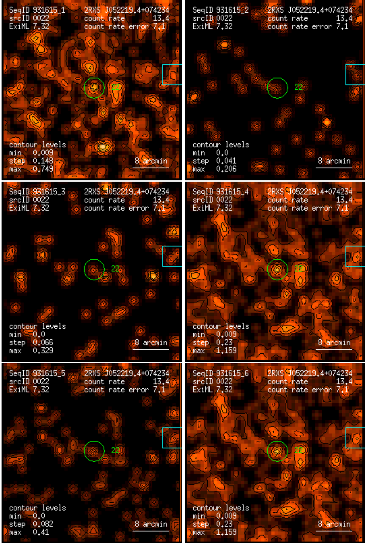
Figure 22: RASS 931615: detection 0022: band rate images, Gaussian filter: (1) PSPC channels 11 – 41, (2) 52 – 90, (3) 91 – 201, (4) 11 – 235, (5) 52 – 201, (6) 11 – 201. Broad band rates in counts/ks. Band rate contour levels in counts/ks/arcmin 2 .
