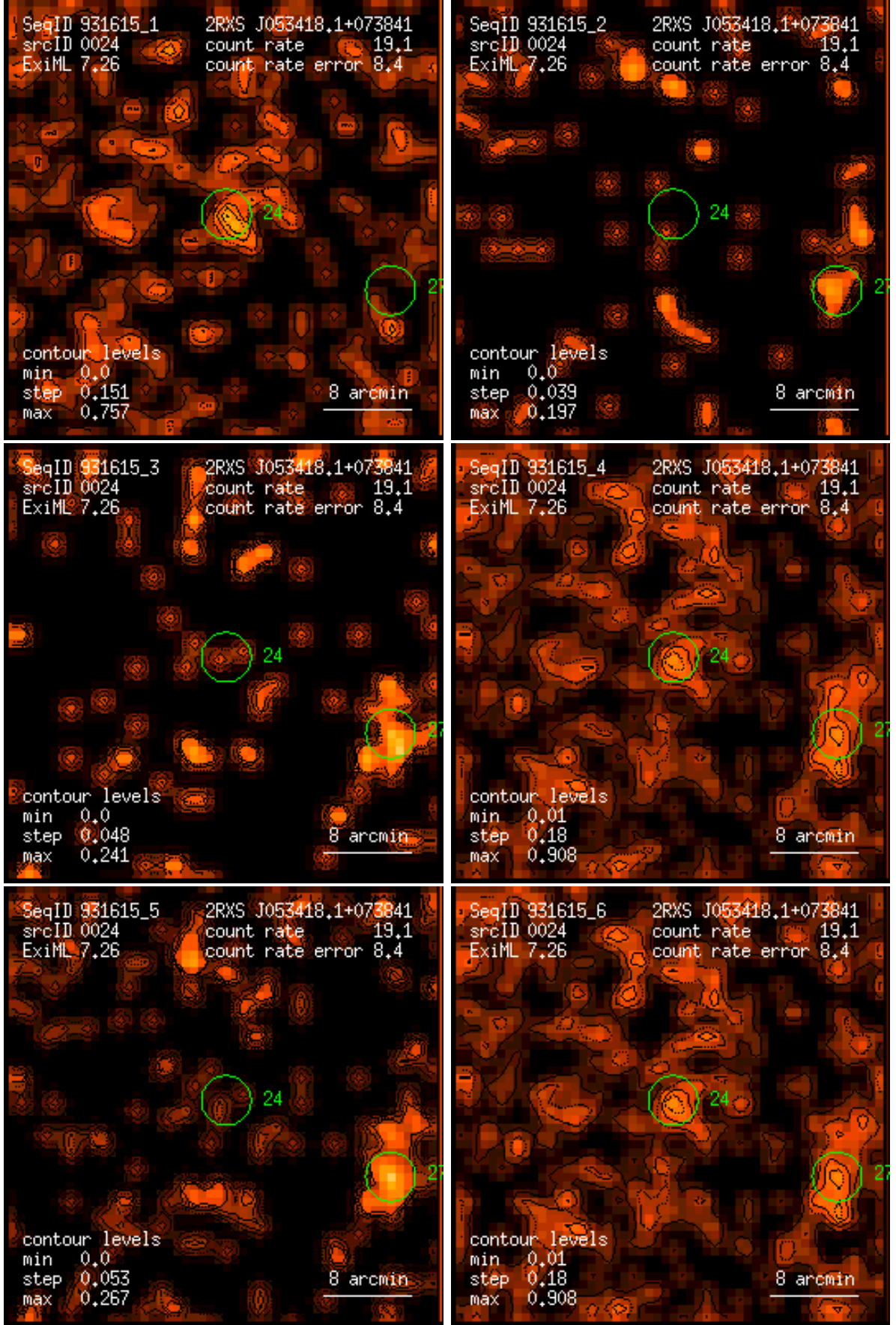
Figure 24: RASS 931615: detection 0024: band rate images, Gaussian filter: (1) PSPC channels 11 – 41, (2) 52 – 90, (3) 91 – 201, (4) 11 – 235, (5) 52 – 201, (6) 11 – 201. Broad band rates in counts/ks. Band rate contour levels in counts/ks/arcmin 2 .
