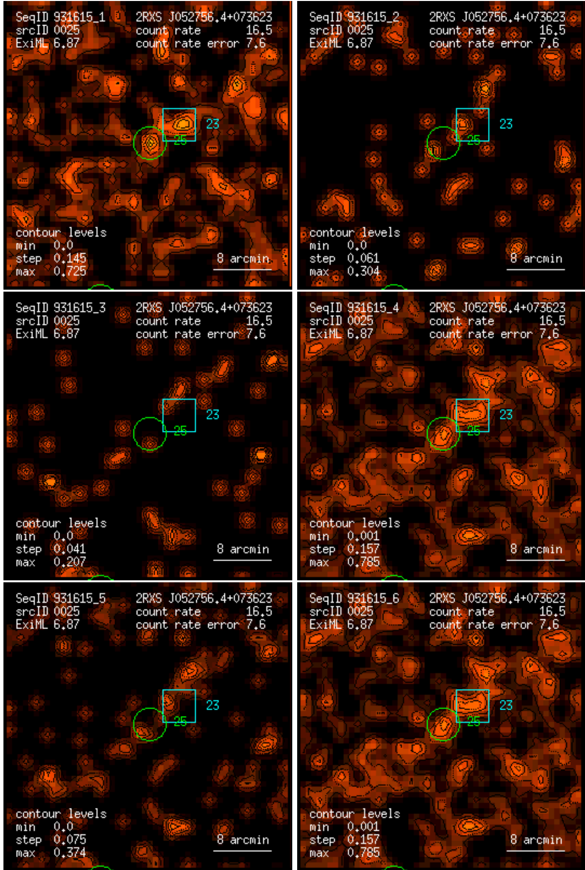
Figure 25: RASS 931615: detection 0025: band rate images, Gaussian filter: (1) PSPC channels 11 – 41, (2) 52 – 90, (3) 91 – 201, (4) 11 – 235, (5) 52 – 201, (6) 11 – 201. Broad band rates in counts/ks. Band rate contour levels in counts/ks/arcmin 2 .
