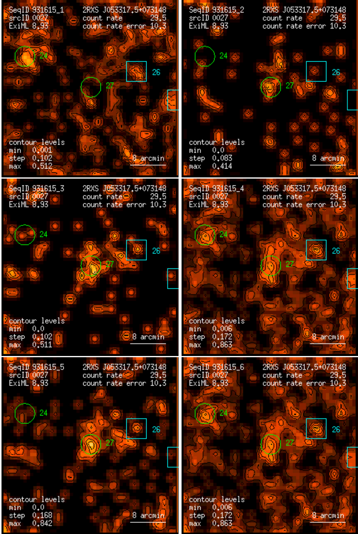
Figure 27: RASS 931615: detection 0027: band rate images, Gaussian filter: (1) PSPC channels 11 – 41, (2) 52 – 90, (3) 91 – 201, (4) 11 – 235, (5) 52 – 201, (6) 11 – 201. Broad band rates in counts/ks. Band rate contour levels in counts/ks/arcmin 2 .
