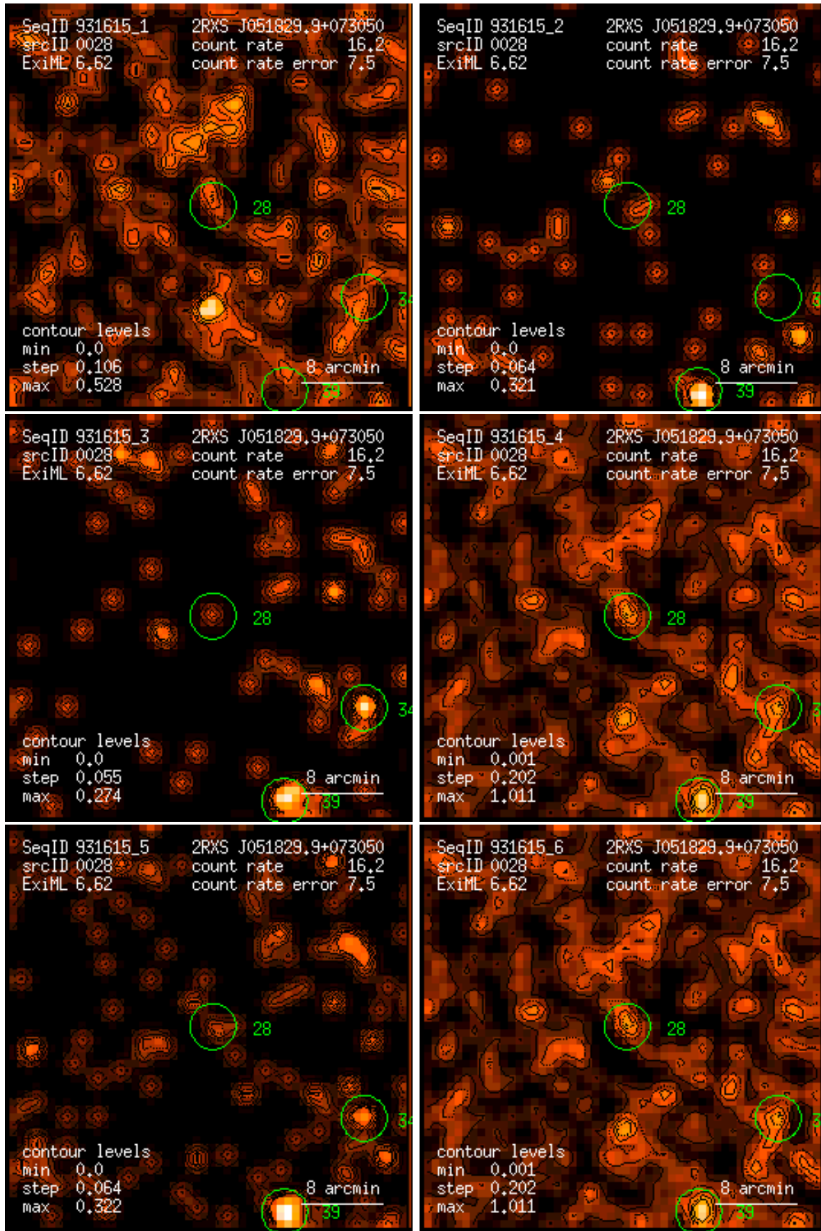
Figure 28: RASS 931615: detection 0028: band rate images, Gaussian filter: (1) PSPC channels 11 – 41, (2) 52 – 90, (3) 91 – 201, (4) 11 – 235, (5) 52 – 201, (6) 11 – 201. Broad band rates in counts/ks. Band rate contour levels in counts/ks/arcmin 2 .
