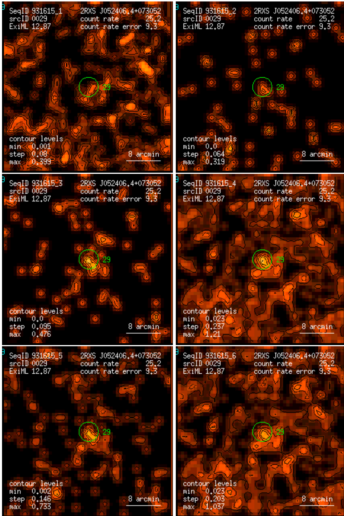
Figure 29: RASS 931615: detection 0029: band rate images, Gaussian filter: (1) PSPC channels 11 – 41, (2) 52 – 90, (3) 91 – 201, (4) 11 – 235, (5) 52 – 201, (6) 11 – 201. Broad band rates in counts/ks. Band rate contour levels in counts/ks/arcmin 2 .
