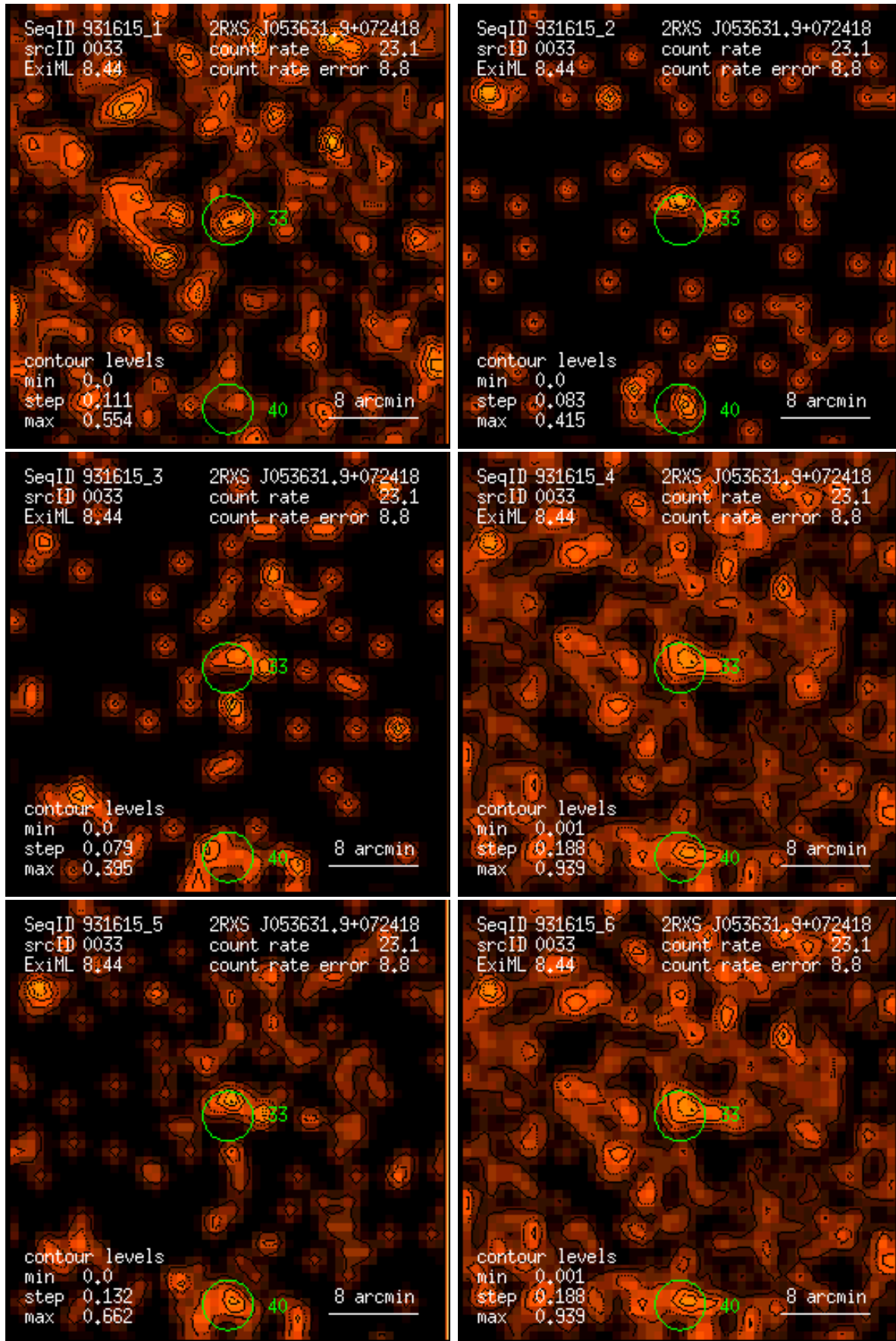
Figure 33: RASS 931615: detection 0033: band rate images, Gaussian filter: (1) PSPC channels 11 – 41, (2) 52 – 90, (3) 91 – 201, (4) 11 – 235, (5) 52 – 201, (6) 11 – 201. Broad band rates in counts/ks. Band rate contour levels in counts/ks/arcmin 2 .
