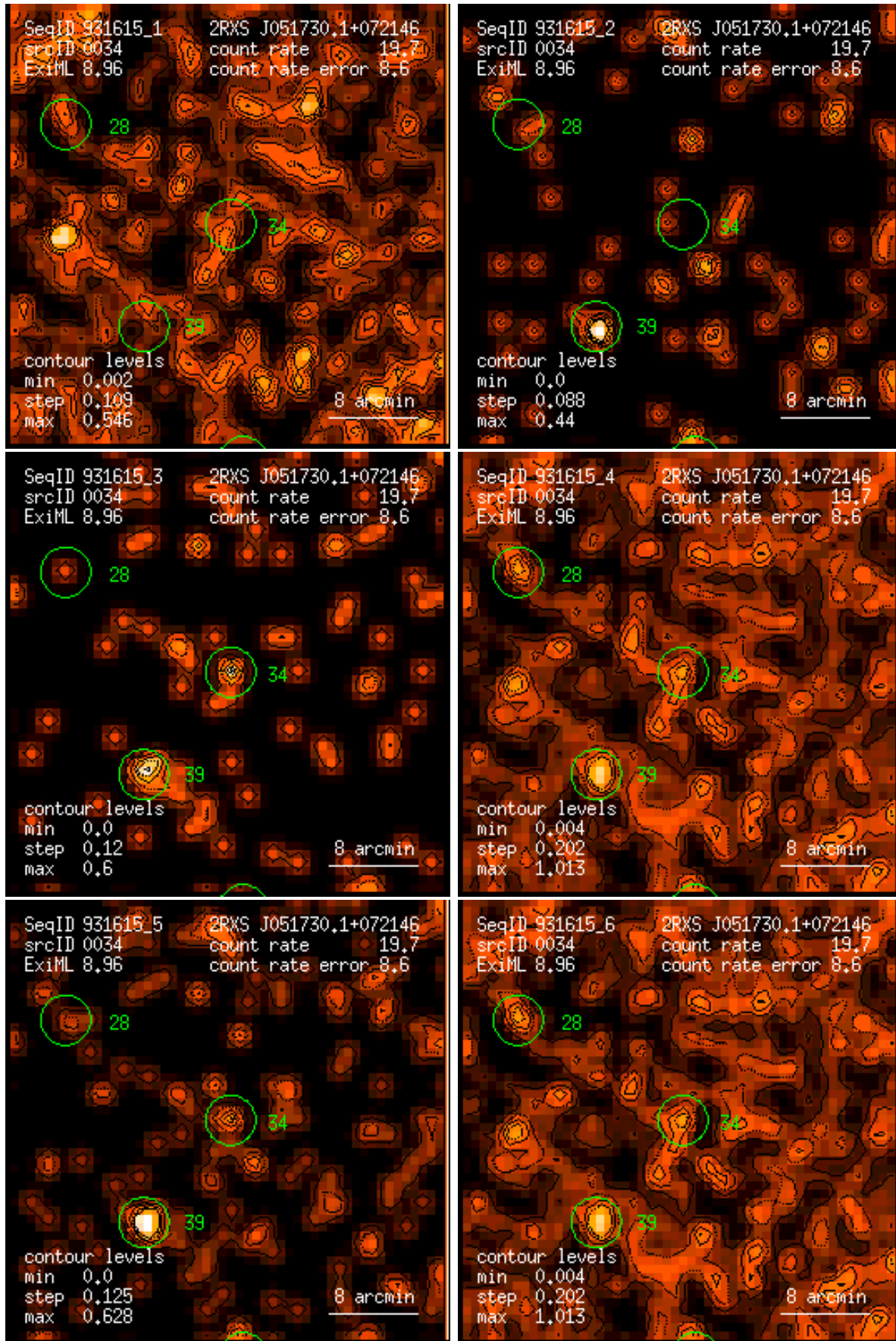
Figure 34: RASS 931615: detection 0034: band rate images, Gaussian filter: (1) PSPC channels 11 – 41, (2) 52 – 90, (3) 91 – 201, (4) 11 – 235, (5) 52 – 201, (6) 11 – 201. Broad band rates in counts/ks. Band rate contour levels in counts/ks/arcmin 2 .
