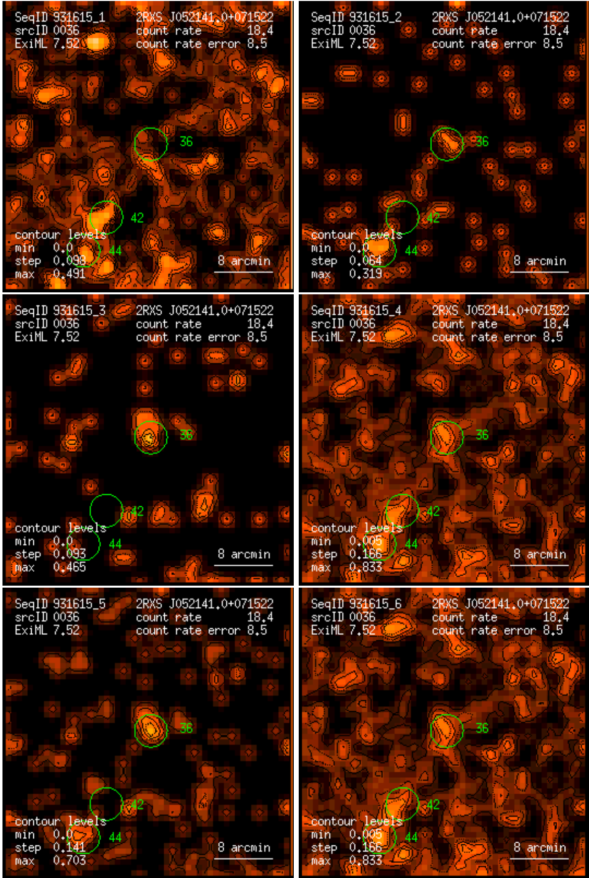
Figure 36: RASS 931615: detection 0036: band rate images, Gaussian filter: (1) PSPC channels 11 – 41, (2) 52 – 90, (3) 91 – 201, (4) 11 – 235, (5) 52 – 201, (6) 11 – 201. Broad band rates in counts/ks. Band rate contour levels in counts/ks/arcmin 2 .
