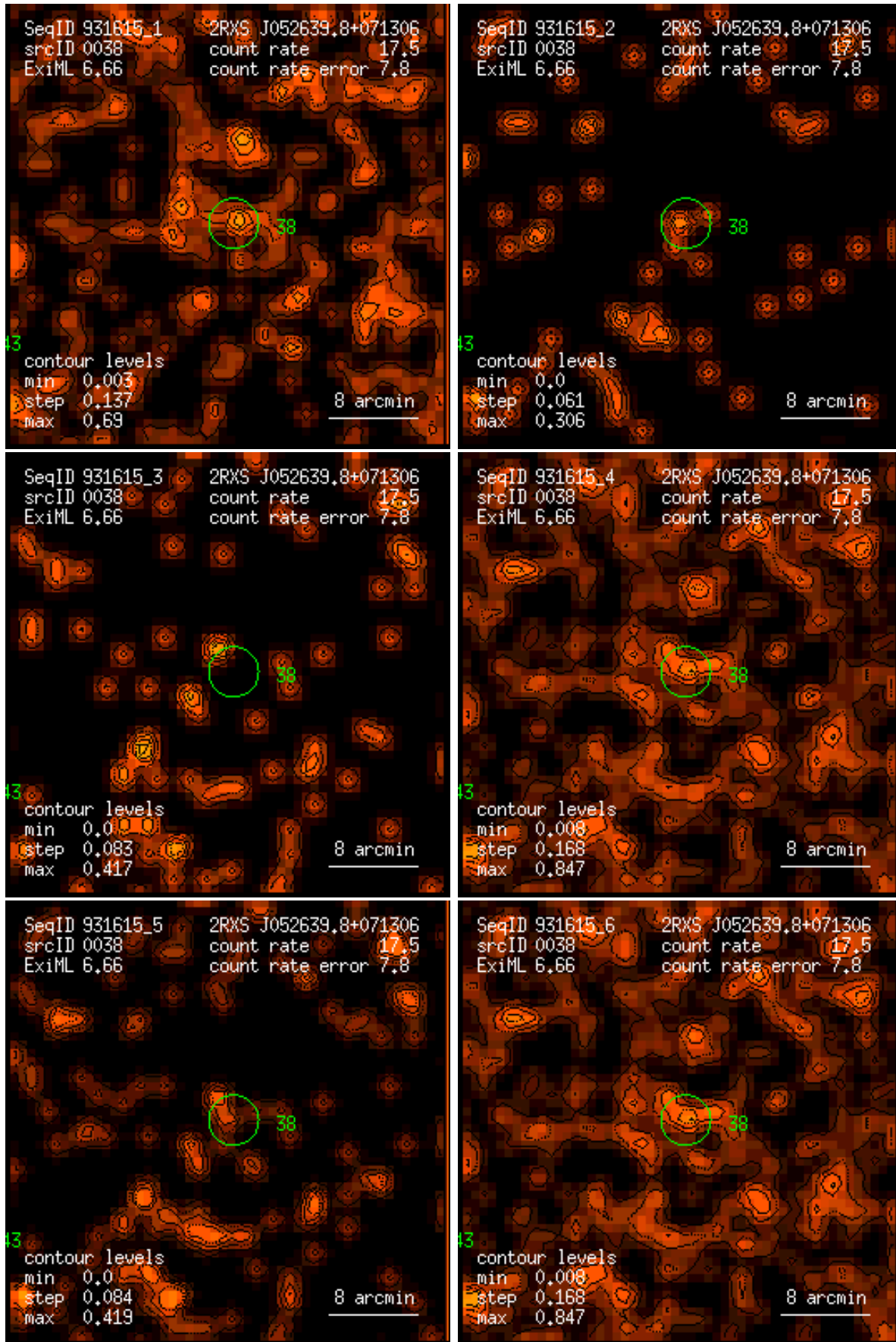
Figure 38: RASS 931615: detection 0038: band rate images, Gaussian filter: (1) PSPC channels 11 – 41, (2) 52 – 90, (3) 91 – 201, (4) 11 – 235, (5) 52 – 201, (6) 11 – 201. Broad band rates in counts/ks. Band rate contour levels in counts/ks/arcmin 2 .
