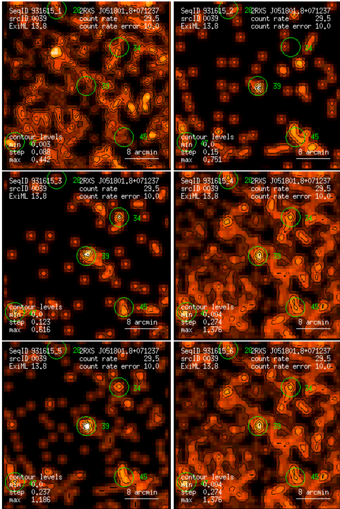
Figure 39: RASS 931615: detection 0039: band rate images, Gaussian filter: (1) PSPC channels 11 – 41, (2) 52 – 90, (3) 91 – 201, (4) 11 – 235, (5) 52 – 201, (6) 11 – 201. Broad band rates in counts/ks. Band rate contour levels in counts/ks/arcmin 2 .
