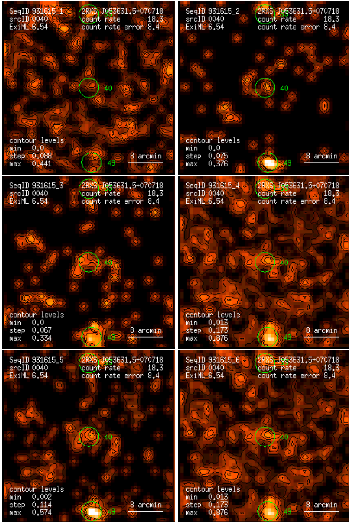
Figure 40: RASS 931615: detection 0040: band rate images, Gaussian filter: (1) PSPC channels 11 – 41, (2) 52 – 90, (3) 91 – 201, (4) 11 – 235, (5) 52 – 201, (6) 11 – 201. Broad band rates in counts/ks. Band rate contour levels in counts/ks/arcmin 2 .
