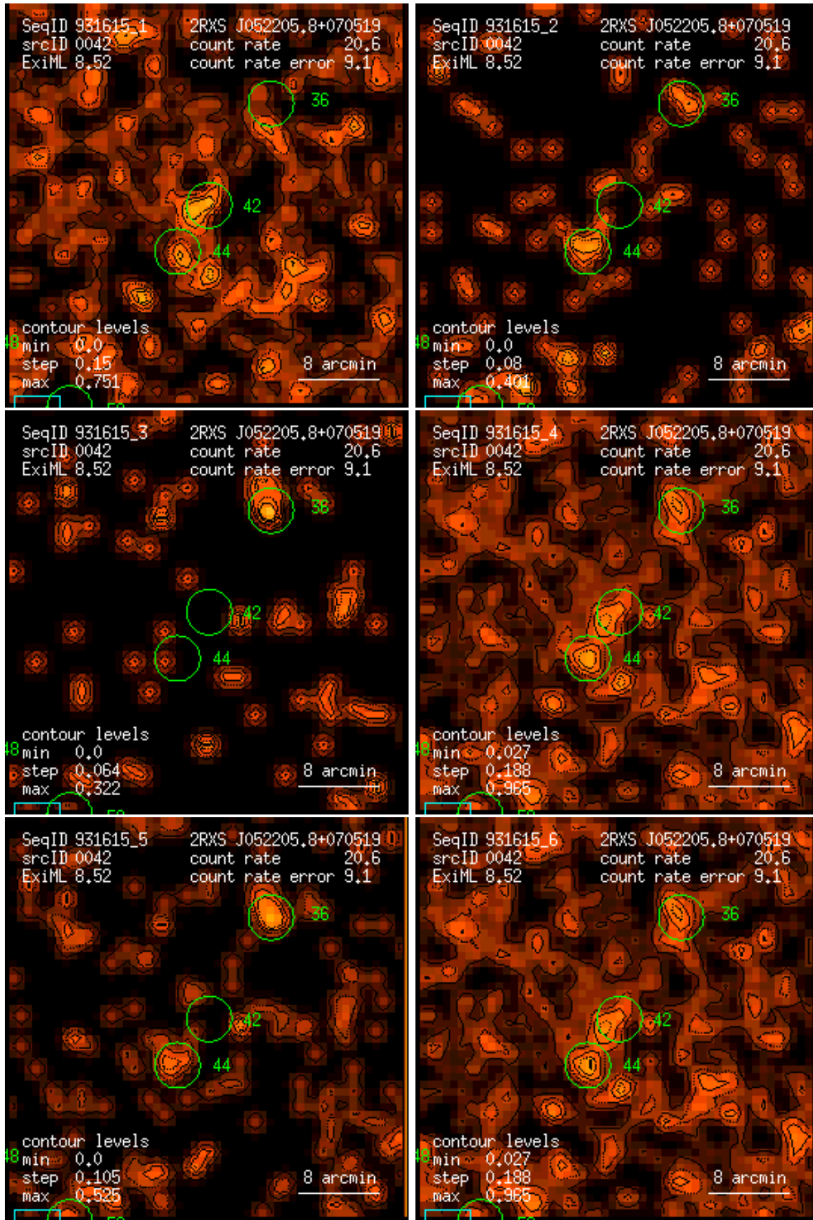
Figure 42: RASS 931615: detection 0042: band rate images, Gaussian filter: (1) PSPC channels 11 – 41, (2) 52 – 90, (3) 91 – 201, (4) 11 – 235, (5) 52 – 201, (6) 11 – 201. Broad band rates in counts/ks. Band rate contour levels in counts/ks/arcmin 2 .
