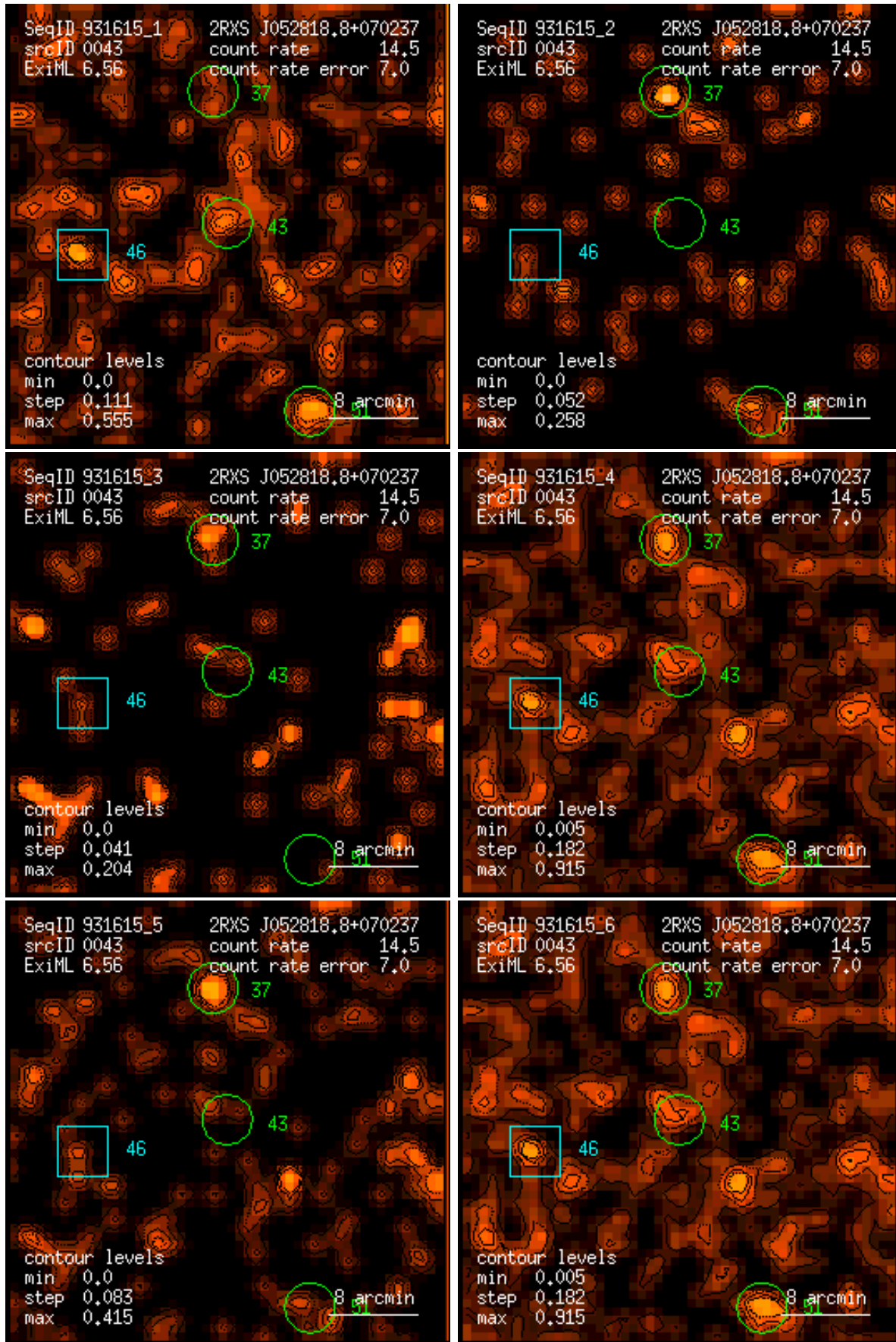
Figure 43: RASS 931615: detection 0043: band rate images, Gaussian filter: (1) PSPC channels 11 – 41, (2) 52 – 90, (3) 91 – 201, (4) 11 – 235, (5) 52 – 201, (6) 11 – 201. Broad band rates in counts/ks. Band rate contour levels in counts/ks/arcmin 2 .
