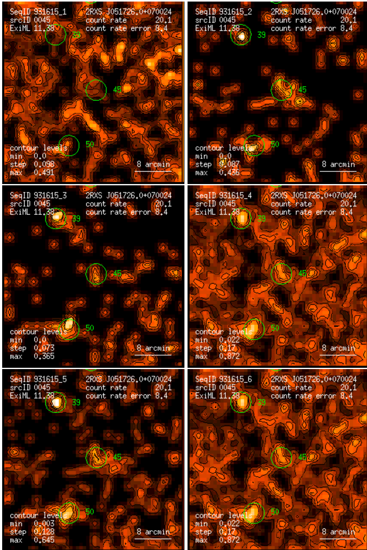
Figure 45: RASS 931615: detection 0045: band rate images, Gaussian filter: (1) PSPC channels 11 – 41, (2) 52 – 90, (3) 91 – 201, (4) 11 – 235, (5) 52 – 201, (6) 11 – 201. Broad band rates in counts/ks. Band rate contour levels in counts/ks/arcmin 2 .
