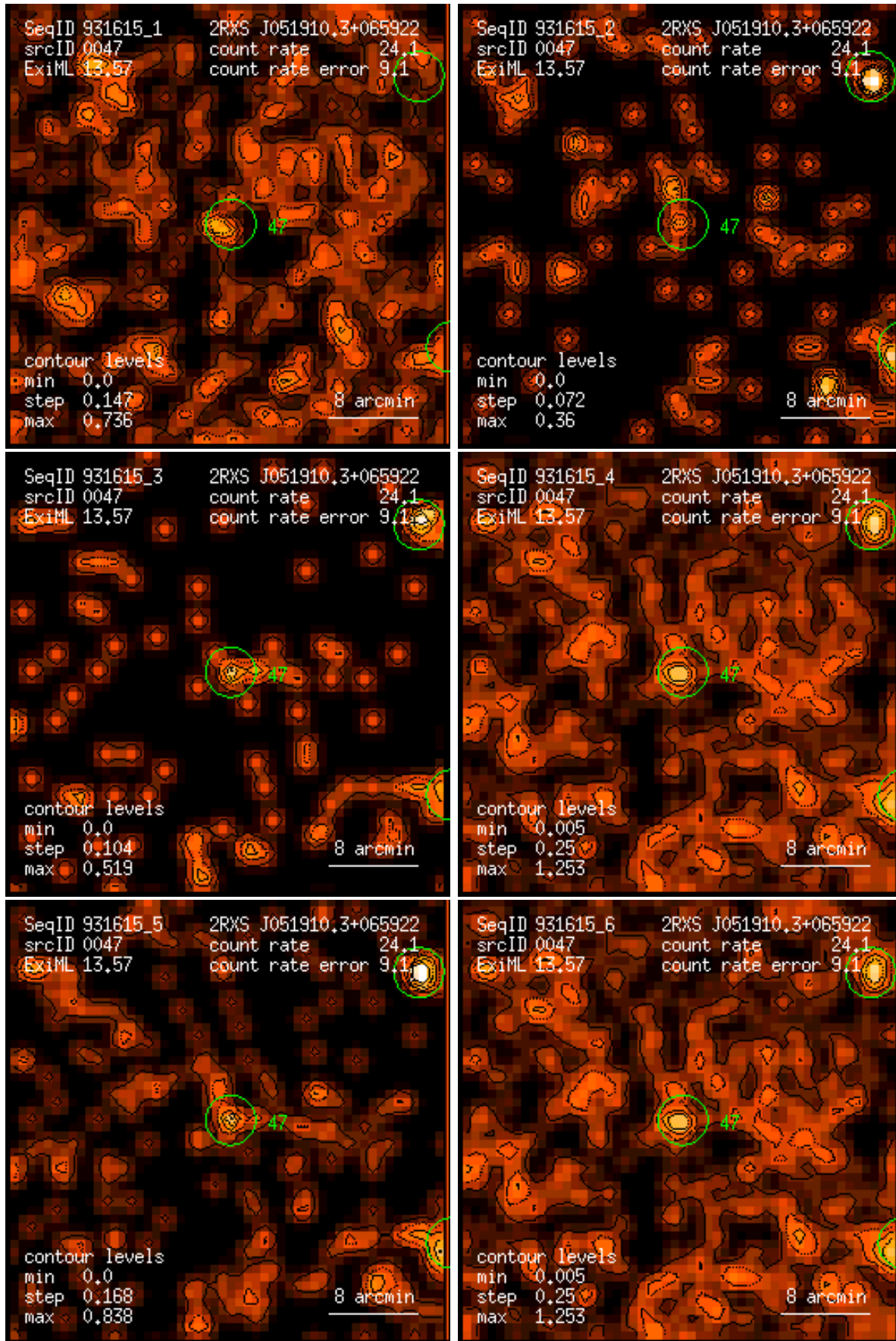
Figure 47: RASS 931615: detection 0047: band rate images, Gaussian filter: (1) PSPC channels 11 – 41, (2) 52 – 90, (3) 91 – 201, (4) 11 – 235, (5) 52 – 201, (6) 11 – 201. Broad band rates in counts/ks. Band rate contour levels in counts/ks/arcmin 2 .
