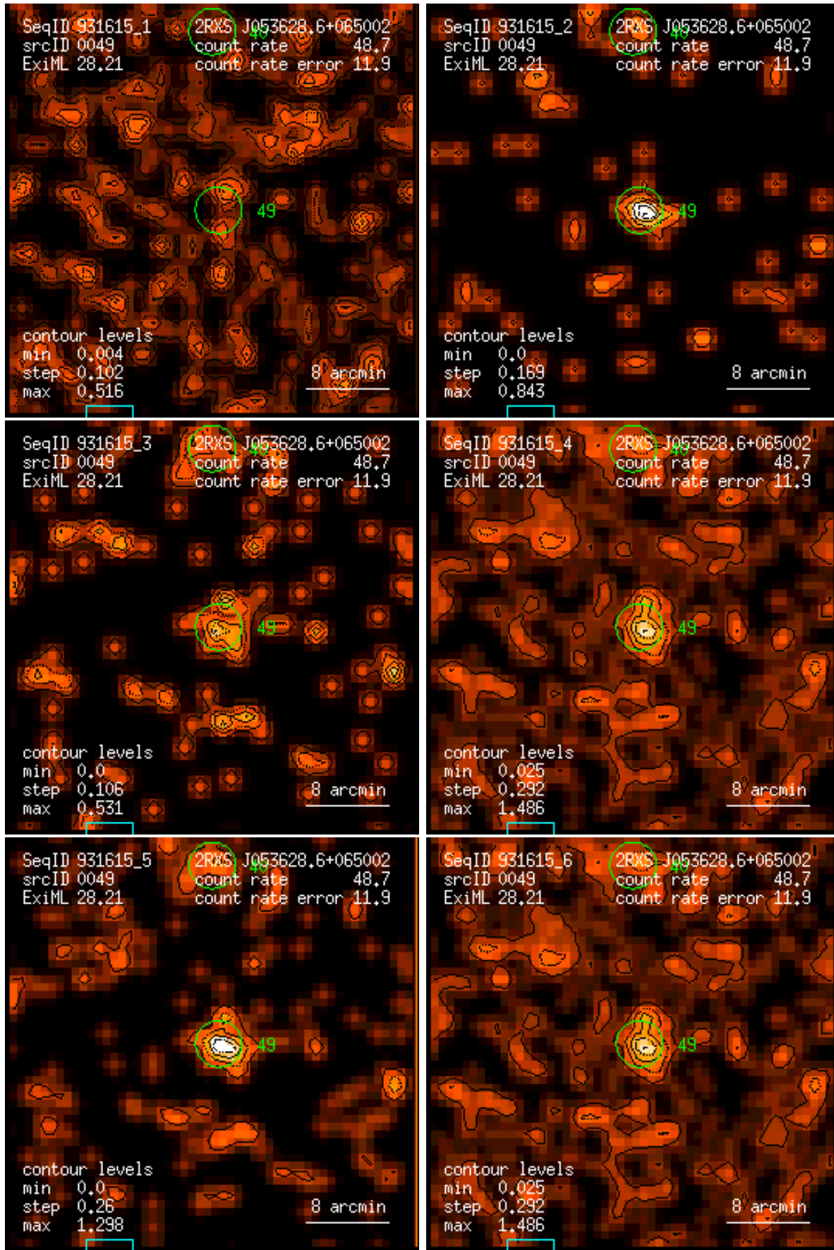
Figure 49: RASS 931615: detection 0049: band rate images, Gaussian filter: (1) PSPC channels 11 – 41, (2) 52 – 90, (3) 91 – 201, (4) 11 – 235, (5) 52 – 201, (6) 11 – 201. Broad band rates in counts/ks. Band rate contour levels in counts/ks/arcmin 2 .
