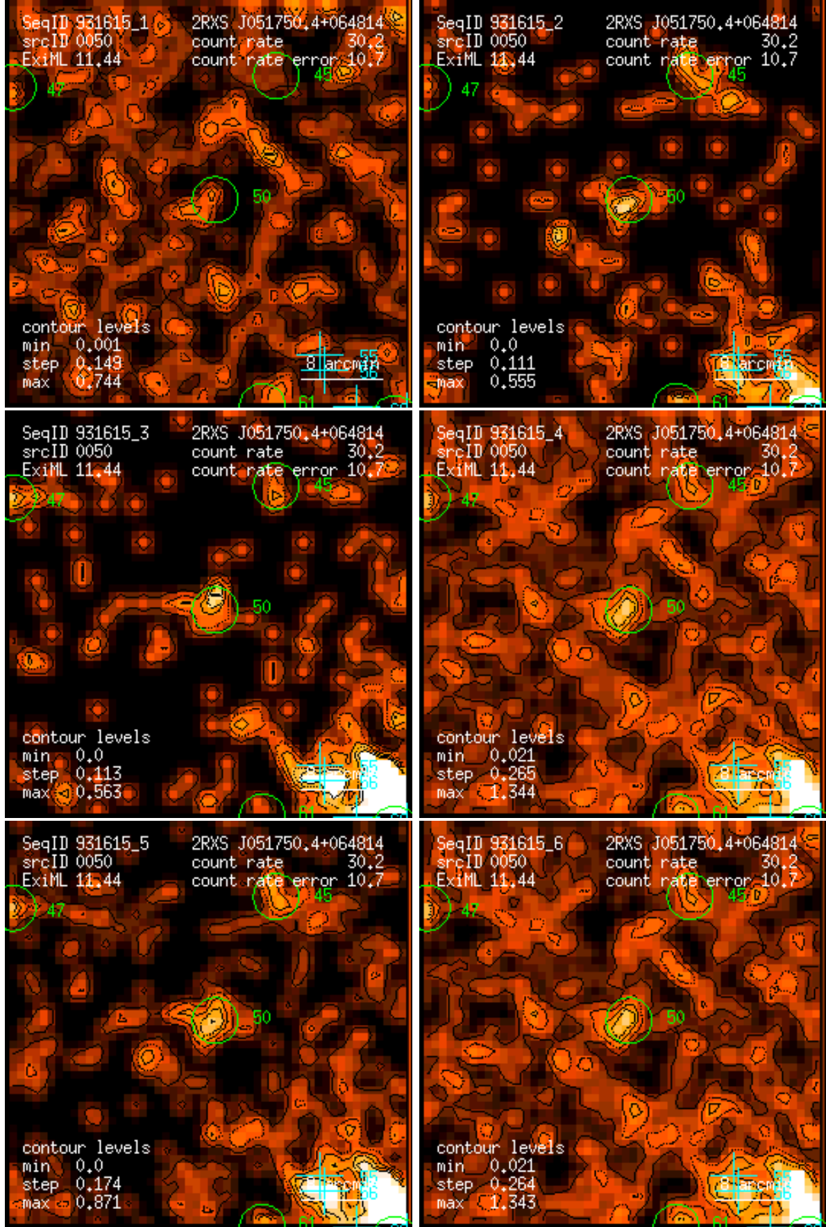
Figure 50: RASS 931615: detection 0050: band rate images, Gaussian filter: (1) PSPC channels 11 – 41, (2) 52 – 90, (3) 91 – 201, (4) 11 – 235, (5) 52 – 201, (6) 11 – 201. Broad band rates in counts/ks. Band rate contour levels in counts/ks/arcmin 2 .
