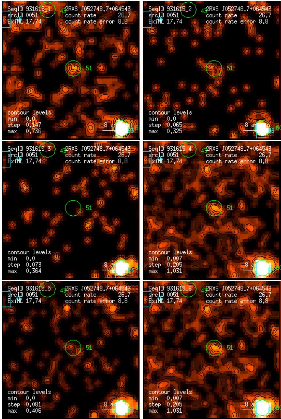
Figure 51: RASS 931615: detection 0051: band rate images, Gaussian filter: (1) PSPC channels 11 – 41, (2) 52 – 90, (3) 91 – 201, (4) 11 – 235, (5) 52 – 201, (6) 11 – 201. Broad band rates in counts/ks. Band rate contour levels in counts/ks/arcmin 2 .
