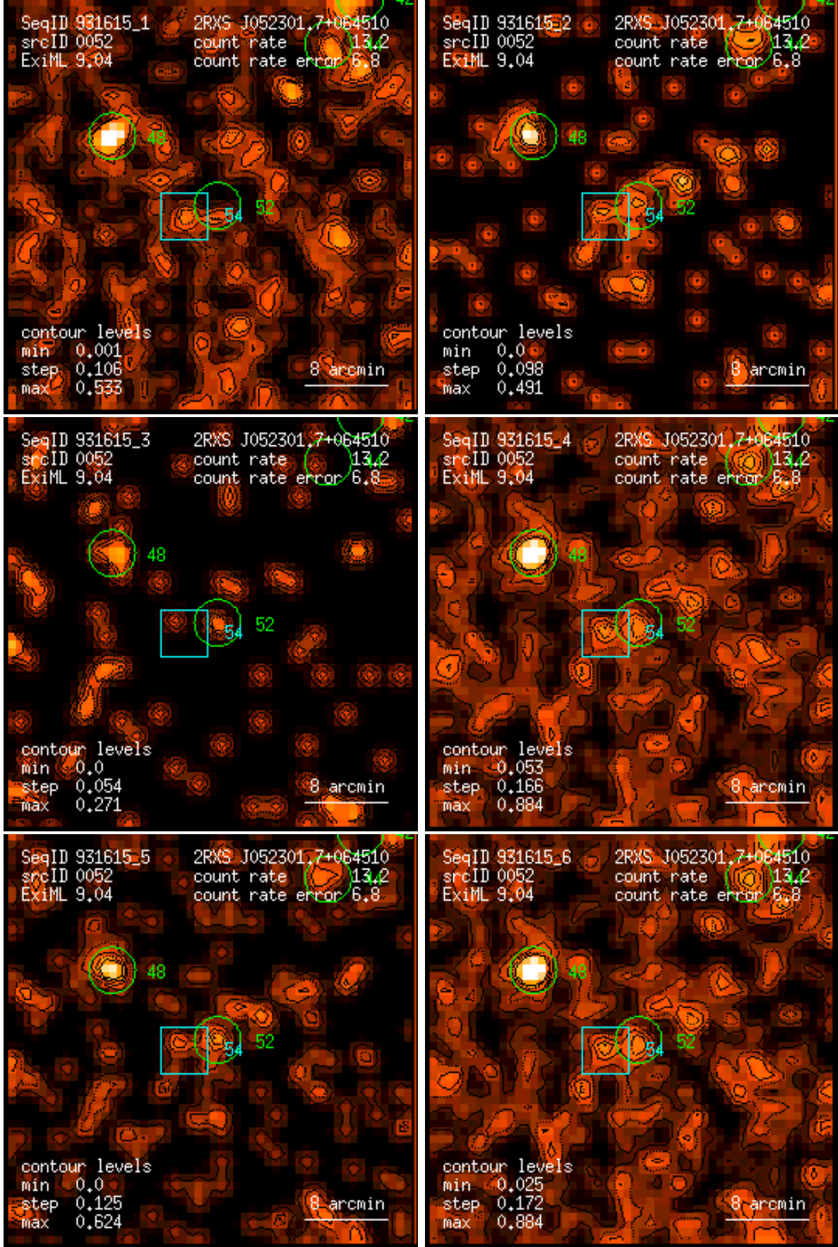
Figure 52: RASS 931615: detection 0052: band rate images, Gaussian filter: (1) PSPC channels 11 – 41, (2) 52 – 90, (3) 91 – 201, (4) 11 – 235, (5) 52 – 201, (6) 11 – 201. Broad band rates in counts/ks. Band rate contour levels in counts/ks/arcmin 2 .
