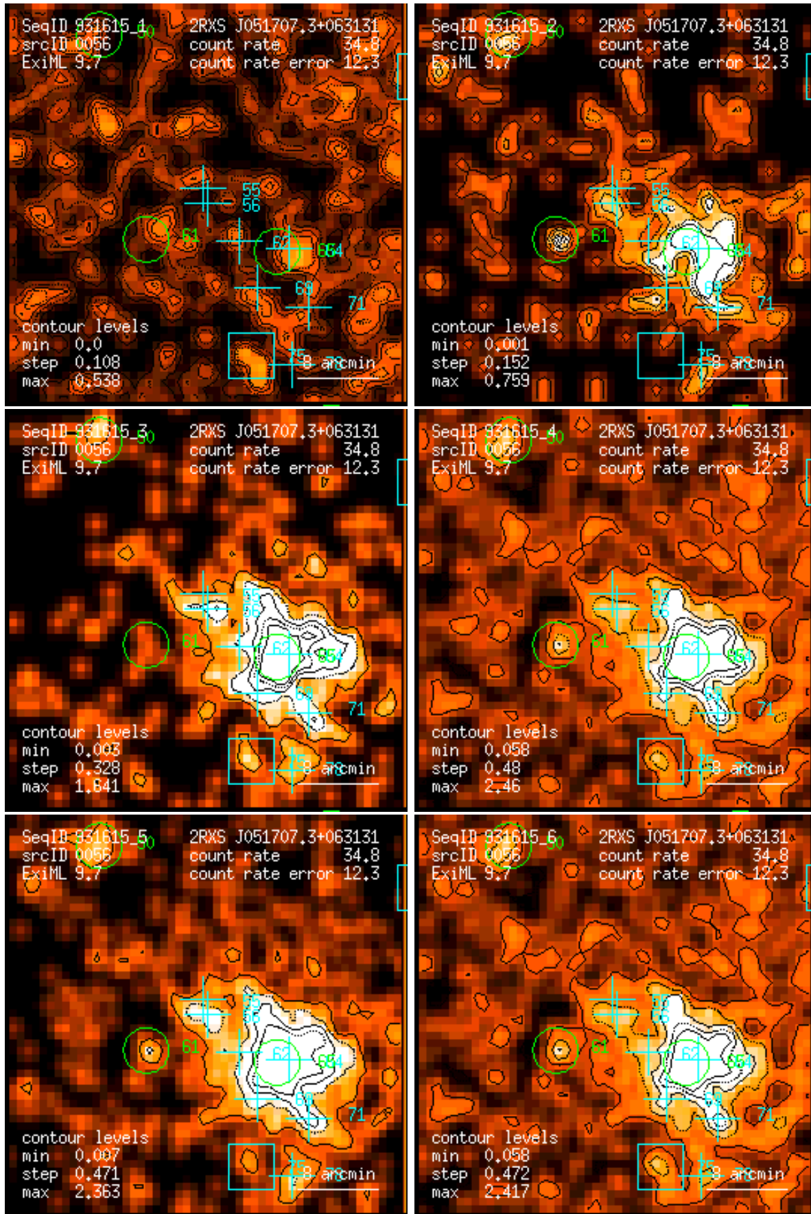
Figure 56: RASS 931615: detection 0056: band rate images, Gaussian filter: (1) PSPC channels 11 – 41, (2) 52 – 90, (3) 91 – 201, (4) 11 – 235, (5) 52 – 201, (6) 11 – 201. Broad band rates in counts/ks. Band rate contour levels in counts/ks/arcmin 2 .
