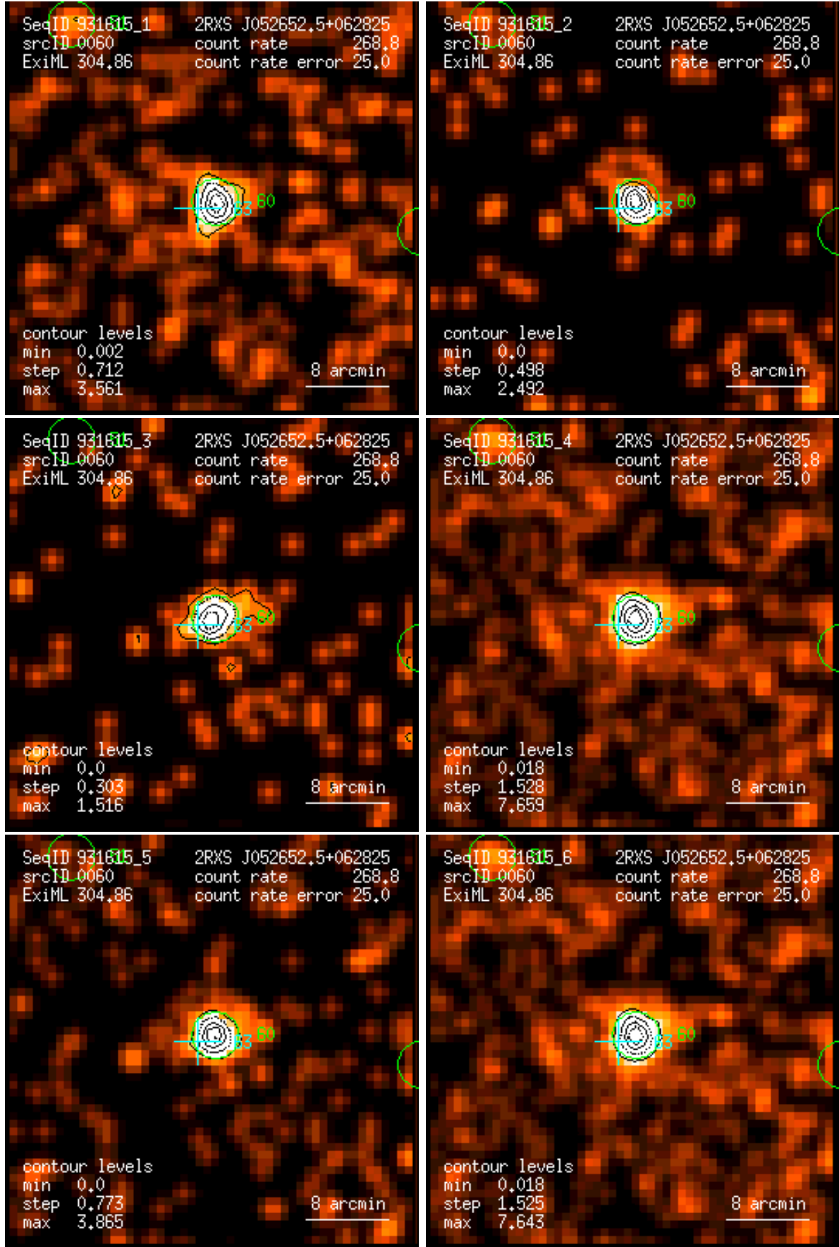
Figure 60: RASS 931615: detection 0060: band rate images, Gaussian filter: (1) PSPC channels 11 – 41, (2) 52 – 90, (3) 91 – 201, (4) 11 – 235, (5) 52 – 201, (6) 11 – 201. Broad band rates in counts/ks. Band rate contour levels in counts/ks/arcmin 2 .
