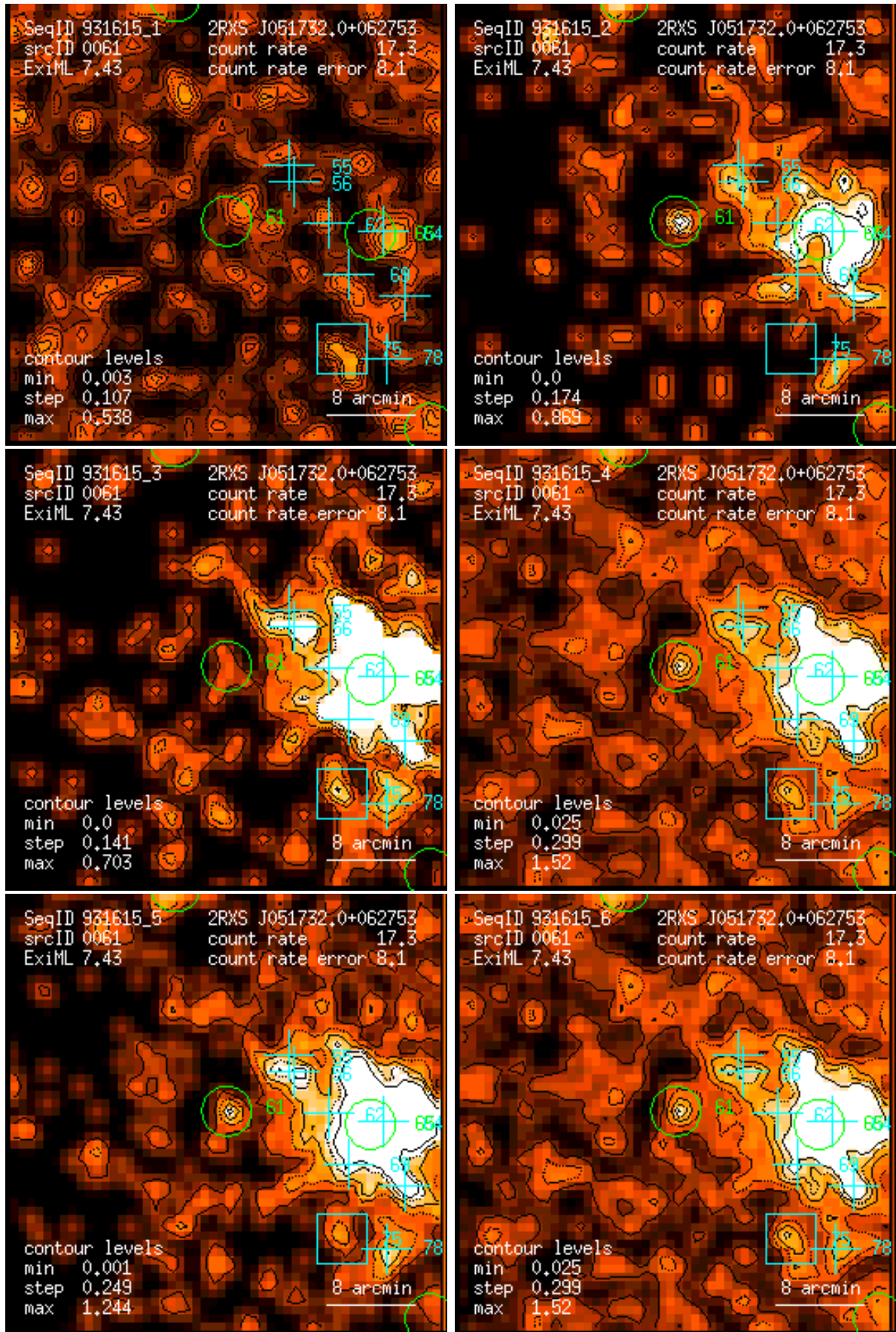
Figure 61: RASS 931615: detection 0061: band rate images, Gaussian filter: (1) PSPC channels 11 – 41, (2) 52 – 90, (3) 91 – 201, (4) 11 – 235, (5) 52 – 201, (6) 11 – 201. Broad band rates in counts/ks. Band rate contour levels in counts/ks/arcmin 2 .
