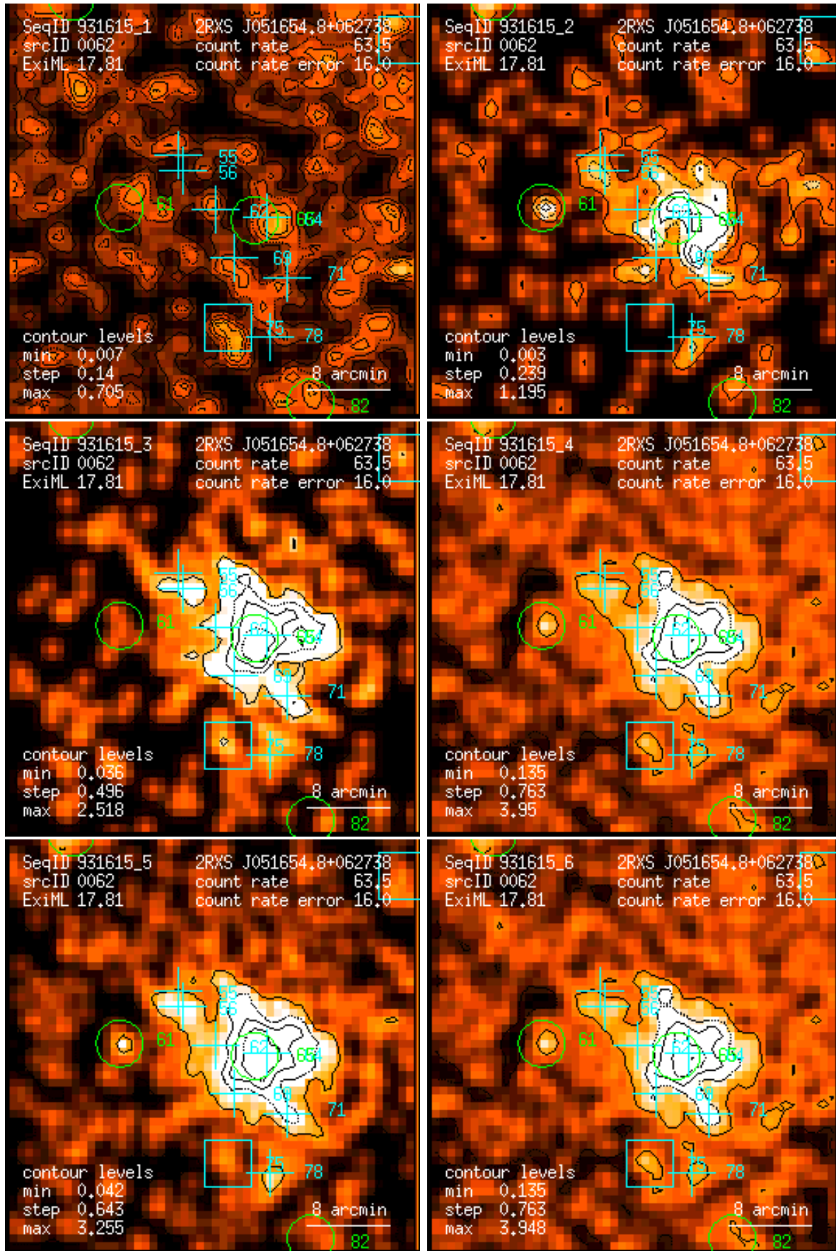
Figure 62: RASS 931615: detection 0062: band rate images, Gaussian filter: (1) PSPC channels 11 – 41, (2) 52 – 90, (3) 91 – 201, (4) 11 – 235, (5) 52 – 201, (6) 11 – 201. Broad band rates in counts/ks. Band rate contour levels in counts/ks/arcmin 2 .
