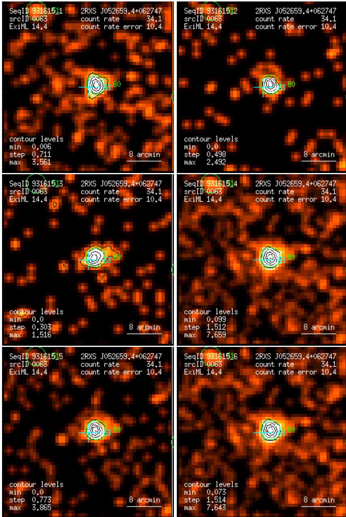
Figure 63: RASS 931615: detection 0063: band rate images, Gaussian filter: (1) PSPC channels 11 – 41, (2) 52 – 90, (3) 91 – 201, (4) 11 – 235, (5) 52 – 201, (6) 11 – 201. Broad band rates in counts/ks. Band rate contour levels in counts/ks/arcmin 2 .
