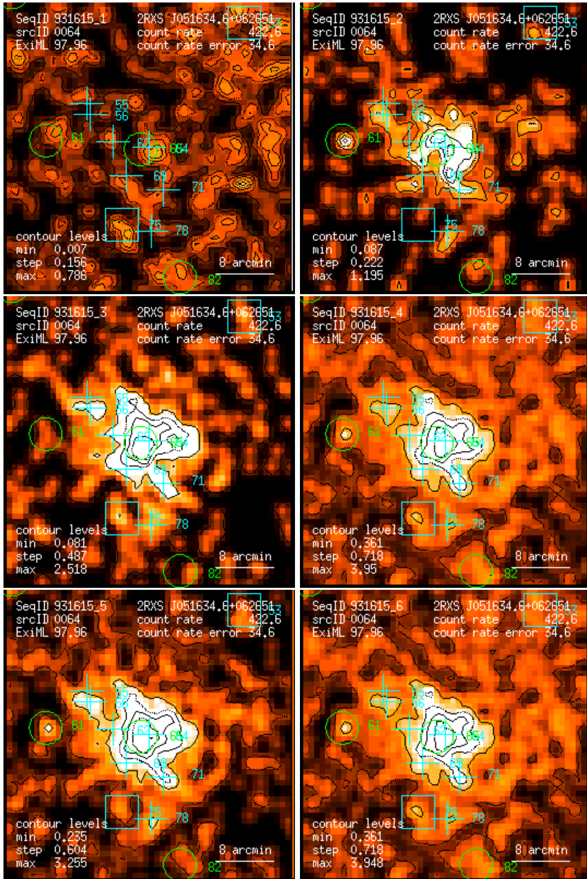
Figure 64: RASS 931615: detection 0064: band rate images, Gaussian filter: (1) PSPC channels 11 – 41, (2) 52 – 90, (3) 91 – 201, (4) 11 – 235, (5) 52 – 201, (6) 11 – 201. Broad band rates in counts/ks. Band rate contour levels in counts/ks/arcmin 2 .
