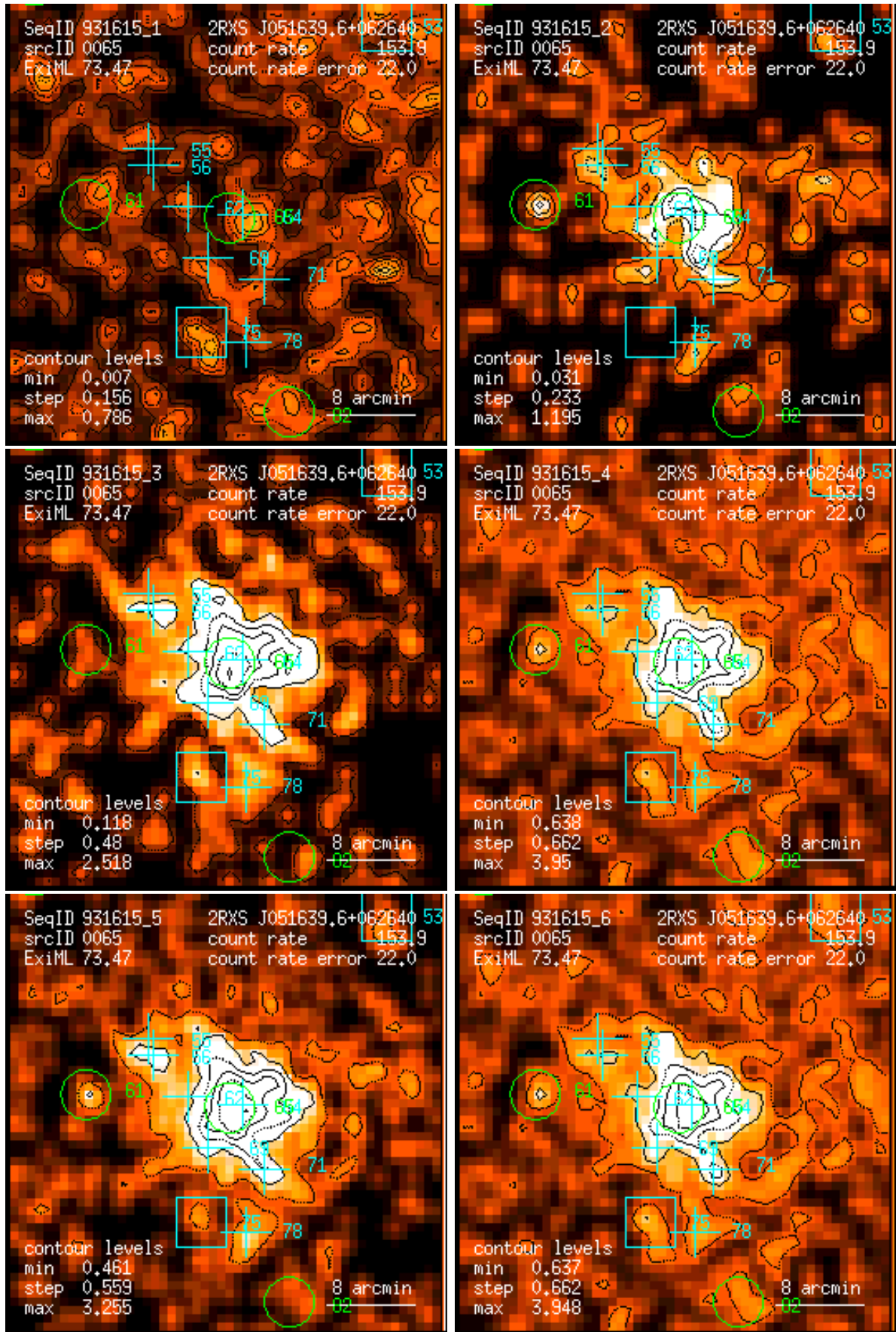
Figure 65: RASS 931615: detection 0065: band rate images, Gaussian filter: (1) PSPC channels 11 – 41, (2) 52 – 90, (3) 91 – 201, (4) 11 – 235, (5) 52 – 201, (6) 11 – 201. Broad band rates in counts/ks. Band rate contour levels in counts/ks/arcmin 2 .
