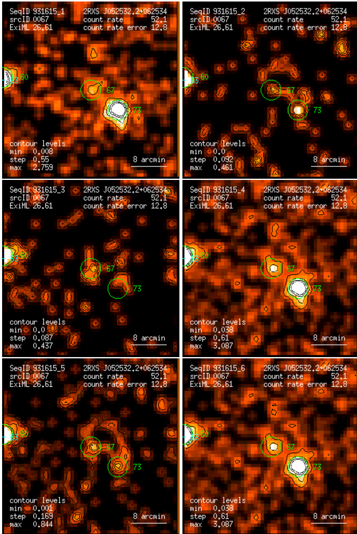
Figure 67: RASS 931615: detection 0067: band rate images, Gaussian filter: (1) PSPC channels 11 – 41, (2) 52 – 90, (3) 91 – 201, (4) 11 – 235, (5) 52 – 201, (6) 11 – 201. Broad band rates in counts/ks. Band rate contour levels in counts/ks/arcmin 2 .
