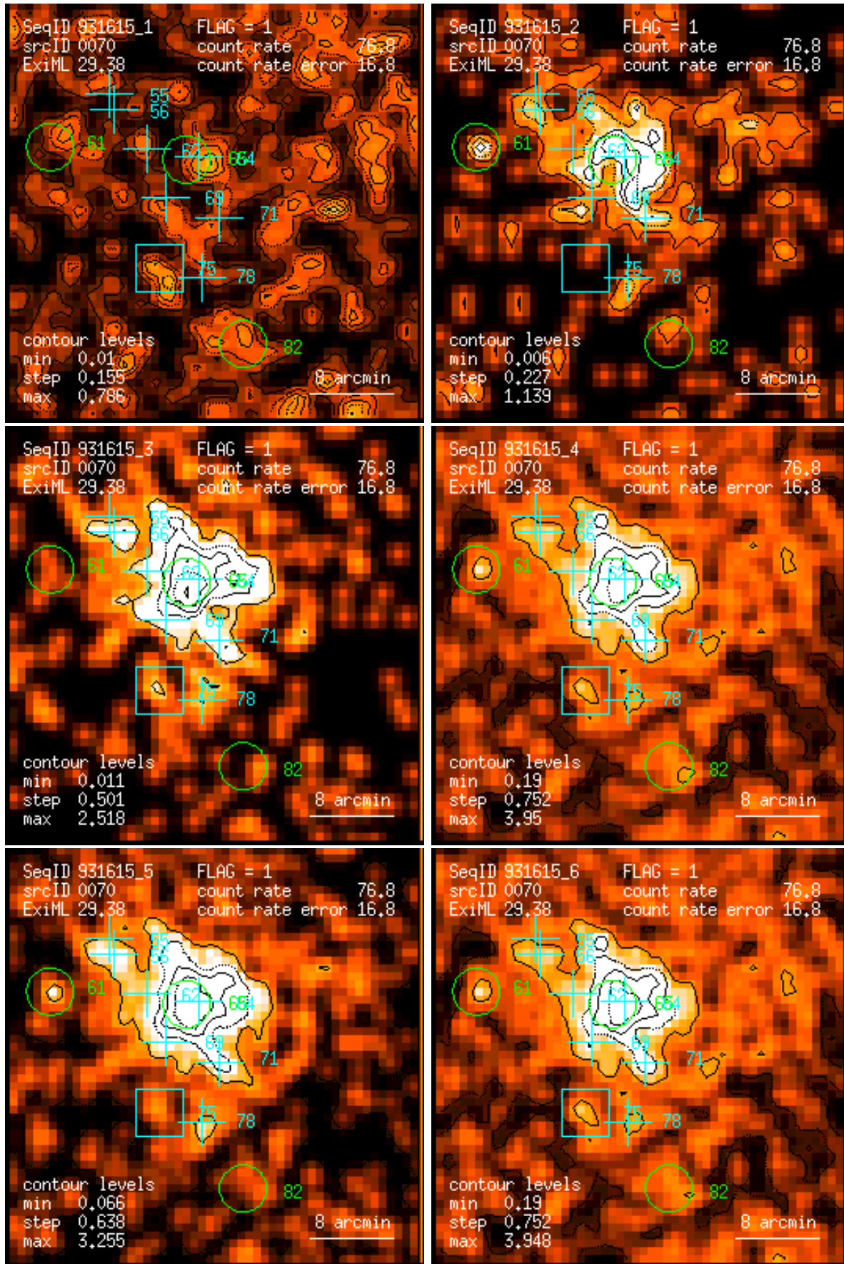
Figure 70: RASS 931615: detection 0070: band rate images, Gaussian filter: (1) PSPC channels 11 – 41, (2) 52 – 90, (3) 91 – 201, (4) 11 – 235, (5) 52 – 201, (6) 11 – 201. Broad band rates in counts/ks. Band rate contour levels in counts/ks/arcmin 2 .
