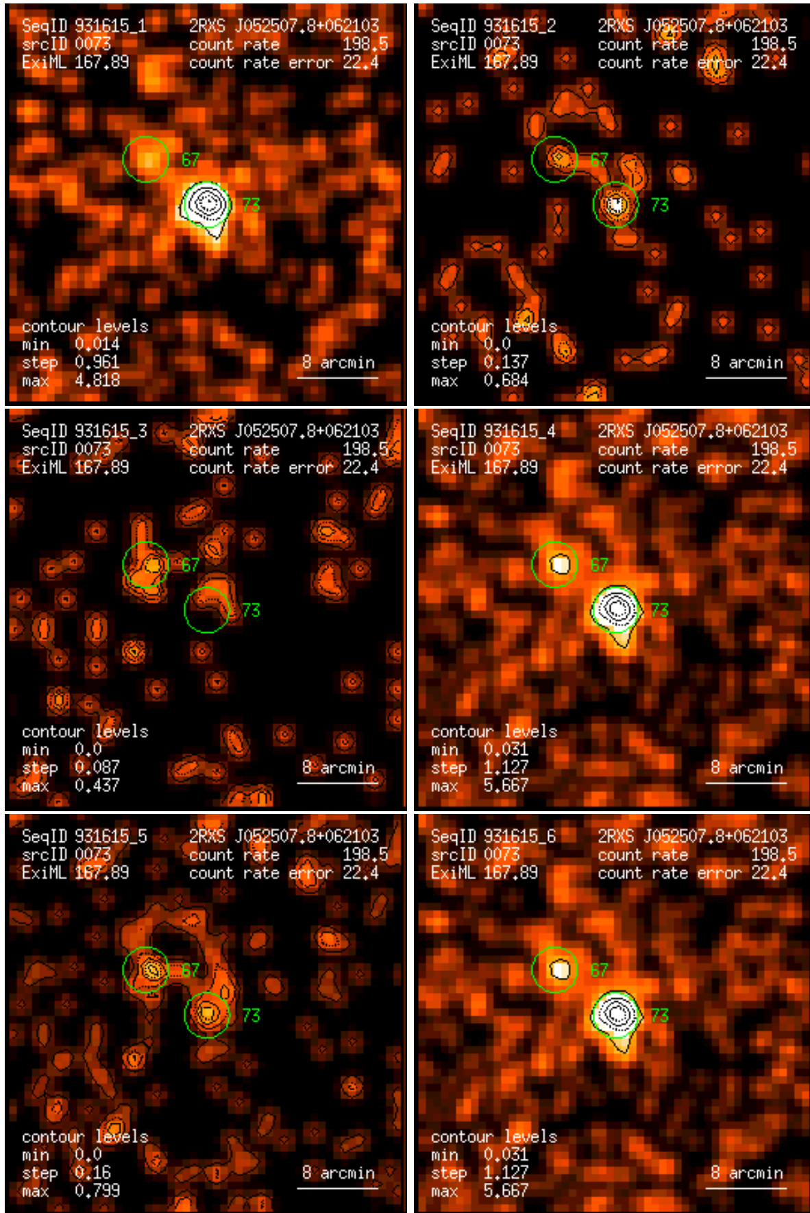
Figure 73: RASS 931615: detection 0073: band rate images, Gaussian filter: (1) PSPC channels 11 – 41, (2) 52 – 90, (3) 91 – 201, (4) 11 – 235, (5) 52 – 201, (6) 11 – 201. Broad band rates in counts/ks. Band rate contour levels in counts/ks/arcmin 2 .
