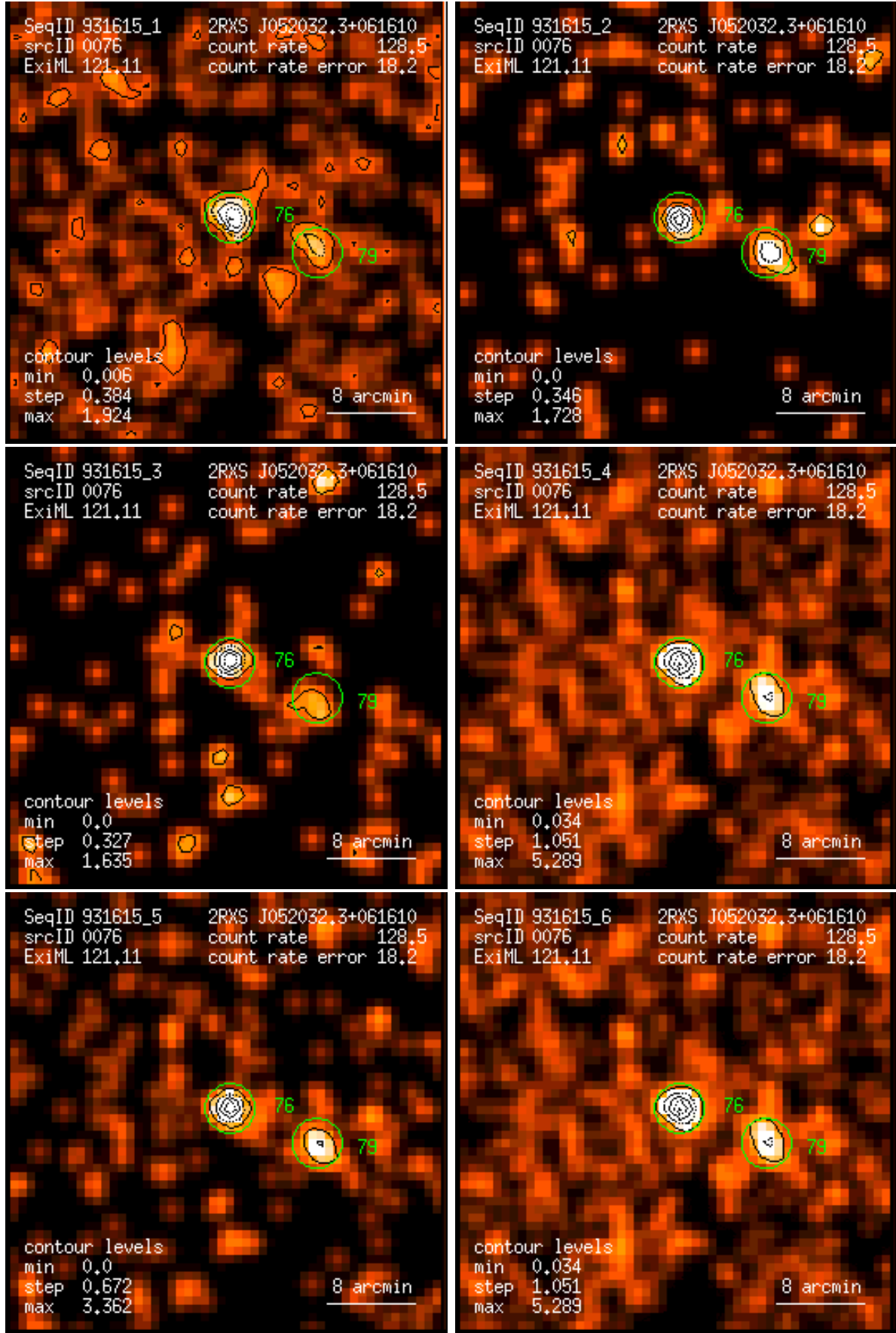
Figure 76: RASS 931615: detection 0076: band rate images, Gaussian filter: (1) PSPC channels 11 – 41, (2) 52 – 90, (3) 91 – 201, (4) 11 – 235, (5) 52 – 201, (6) 11 – 201. Broad band rates in counts/ks. Band rate contour levels in counts/ks/arcmin 2 .
