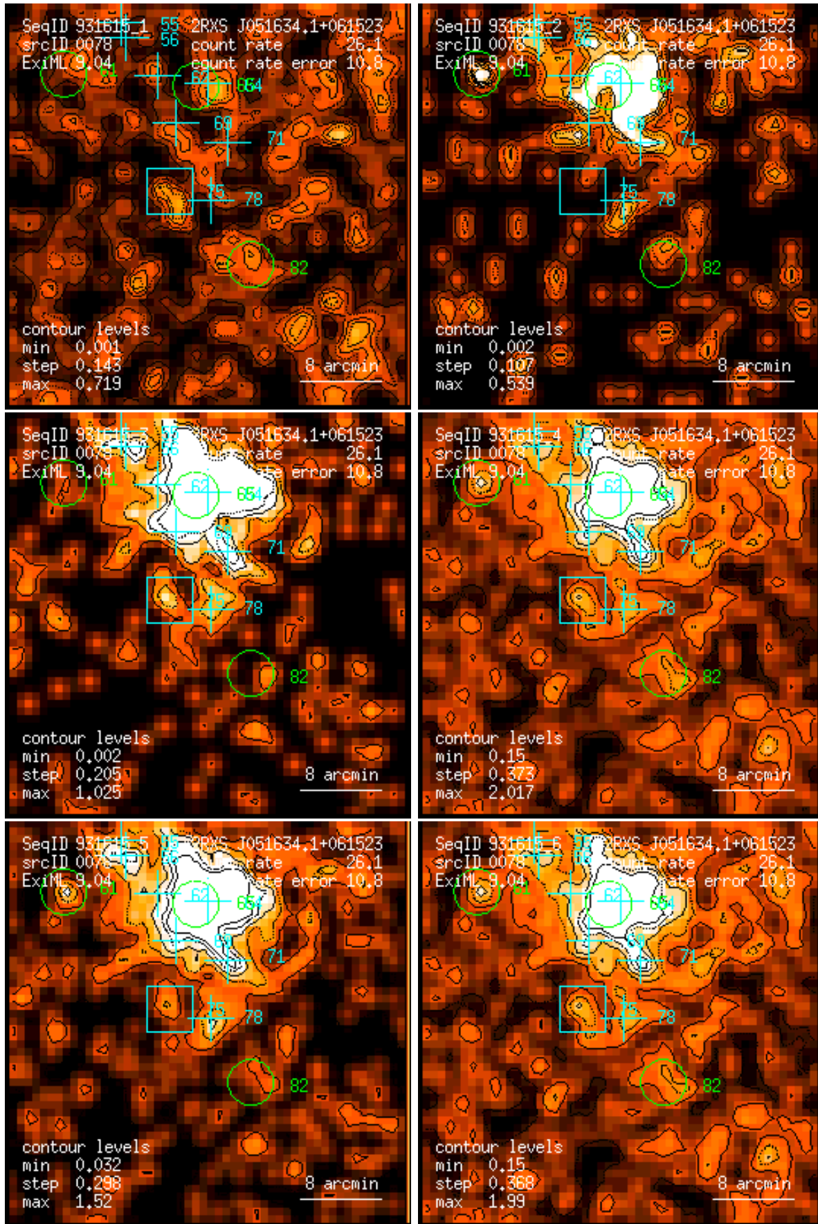
Figure 78: RASS 931615: detection 0078: band rate images, Gaussian filter: (1) PSPC channels 11 – 41, (2) 52 – 90, (3) 91 – 201, (4) 11 – 235, (5) 52 – 201, (6) 11 – 201. Broad band rates in counts/ks. Band rate contour levels in counts/ks/arcmin 2 .
