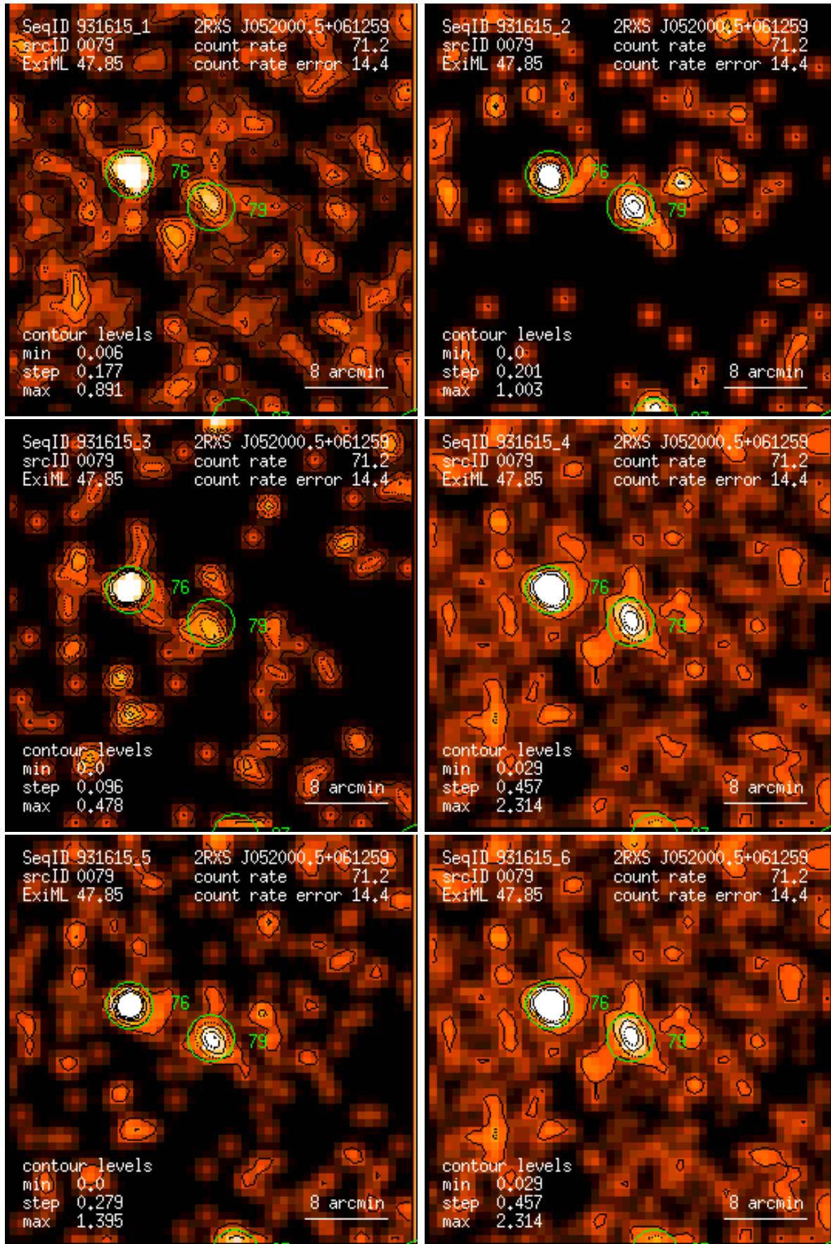
Figure 79: RASS 931615: detection 0079: band rate images, Gaussian filter: (1) PSPC channels 11 – 41, (2) 52 – 90, (3) 91 – 201, (4) 11 – 235, (5) 52 – 201, (6) 11 – 201. Broad band rates in counts/ks. Band rate contour levels in counts/ks/arcmin 2 .
