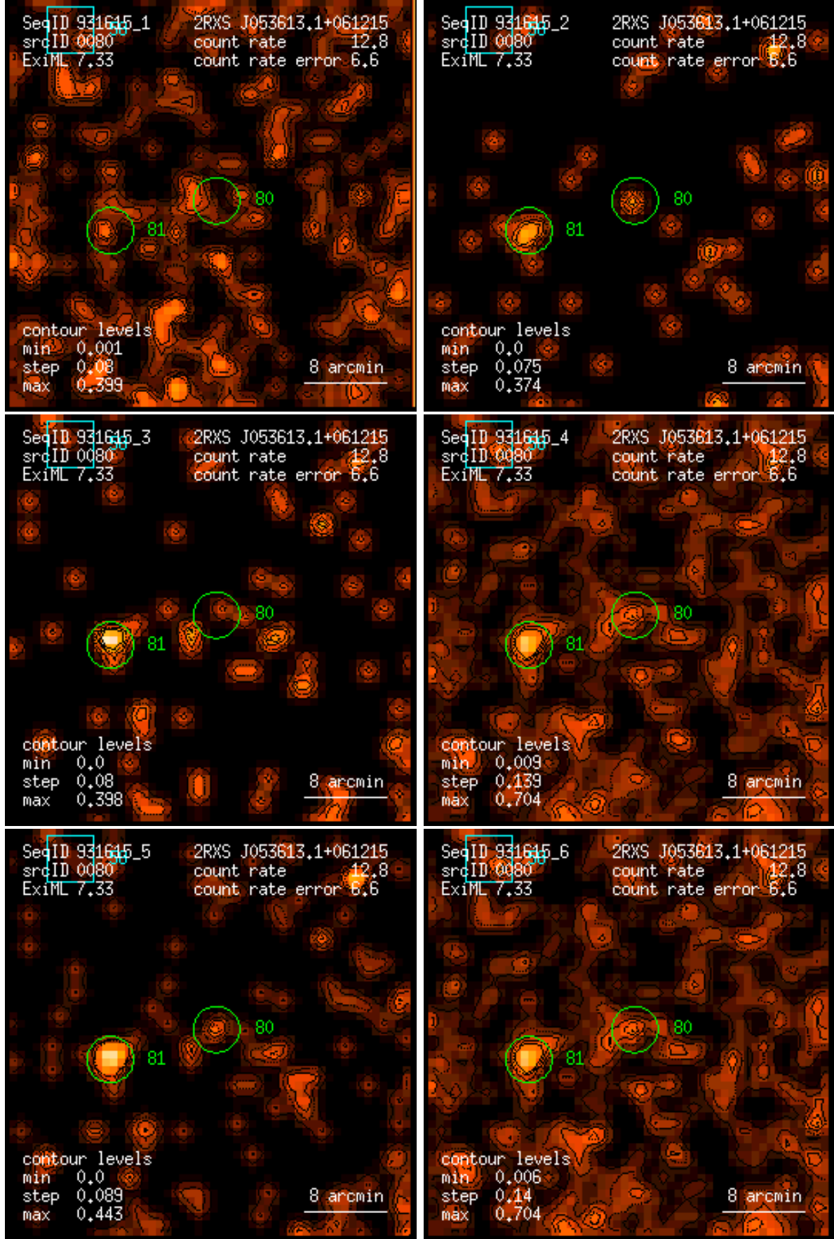
Figure 80: RASS 931615: detection 0080: band rate images, Gaussian filter: (1) PSPC channels 11 – 41, (2) 52 – 90, (3) 91 – 201, (4) 11 – 235, (5) 52 – 201, (6) 11 – 201. Broad band rates in counts/ks. Band rate contour levels in counts/ks/arcmin 2 .
