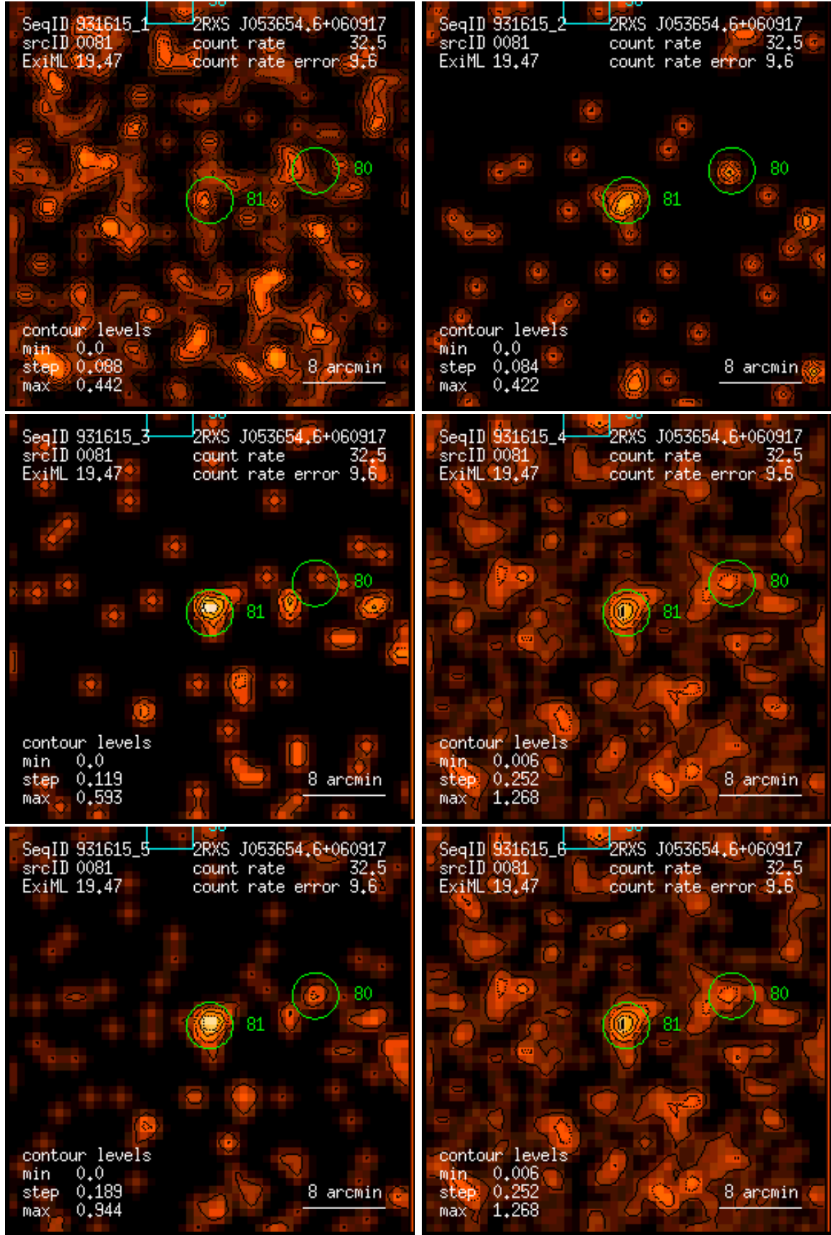
Figure 81: RASS 931615: detection 0081: band rate images, Gaussian filter: (1) PSPC channels 11 – 41, (2) 52 – 90, (3) 91 – 201, (4) 11 – 235, (5) 52 – 201, (6) 11 – 201. Broad band rates in counts/ks. Band rate contour levels in counts/ks/arcmin 2 .
