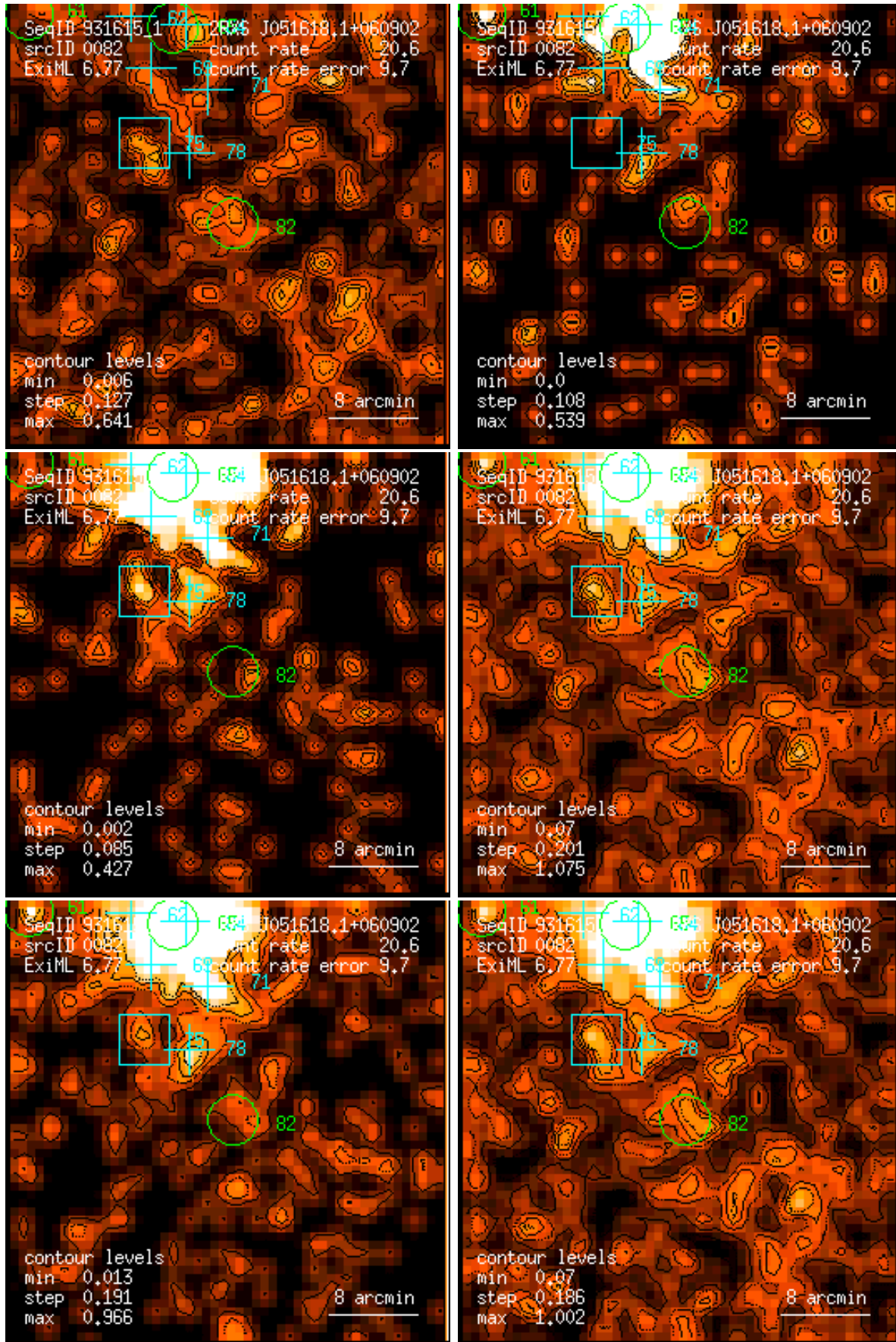
Figure 82: RASS 931615: detection 0082: band rate images, Gaussian filter: (1) PSPC channels 11 – 41, (2) 52 – 90, (3) 91 – 201, (4) 11 – 235, (5) 52 – 201, (6) 11 – 201. Broad band rates in counts/ks. Band rate contour levels in counts/ks/arcmin 2 .
