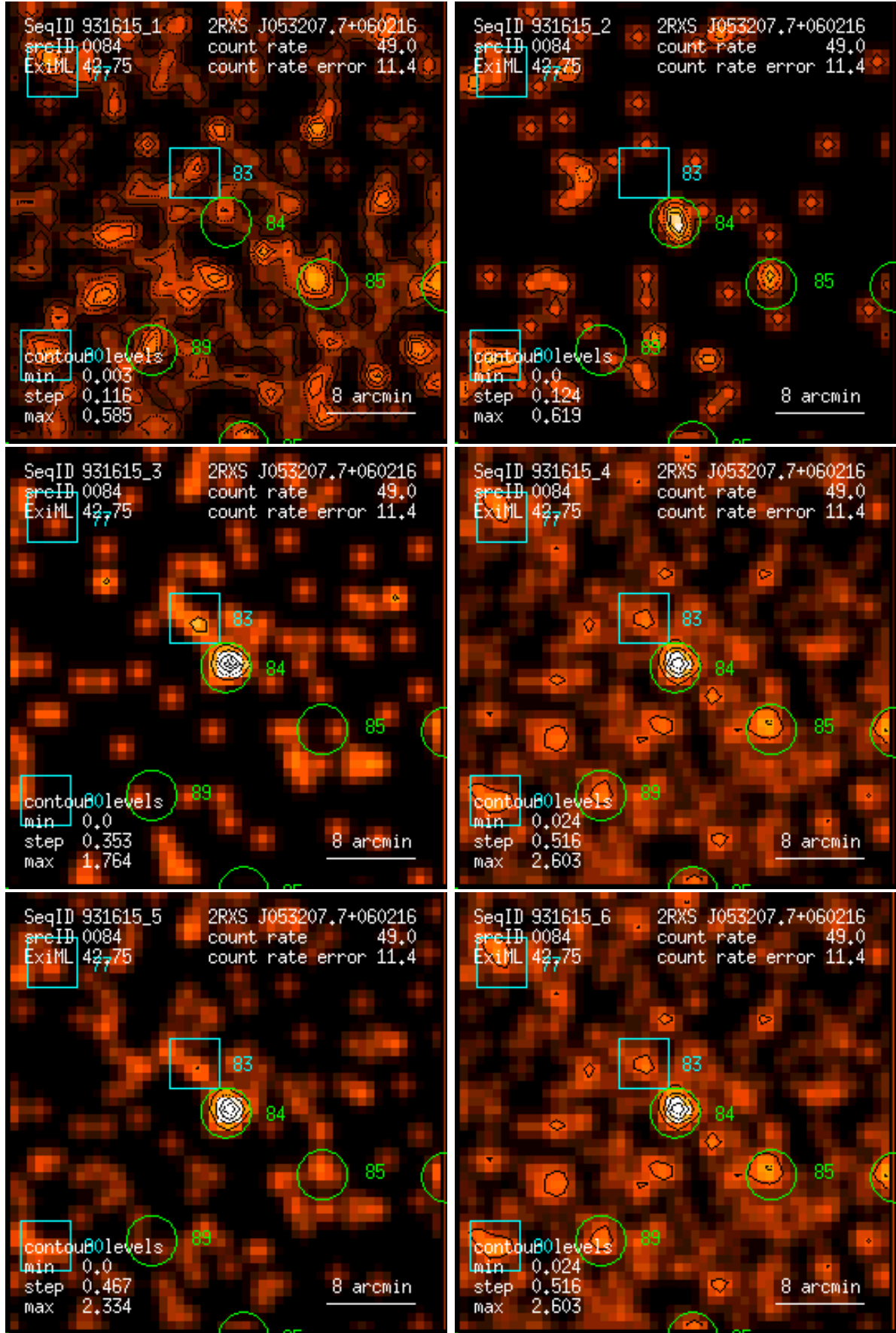
Figure 84: RASS 931615: detection 0084: band rate images, Gaussian filter: (1) PSPC channels 11 – 41, (2) 52 – 90, (3) 91 – 201, (4) 11 – 235, (5) 52 – 201, (6) 11 – 201. Broad band rates in counts/ks. Band rate contour levels in counts/ks/arcmin 2 .
