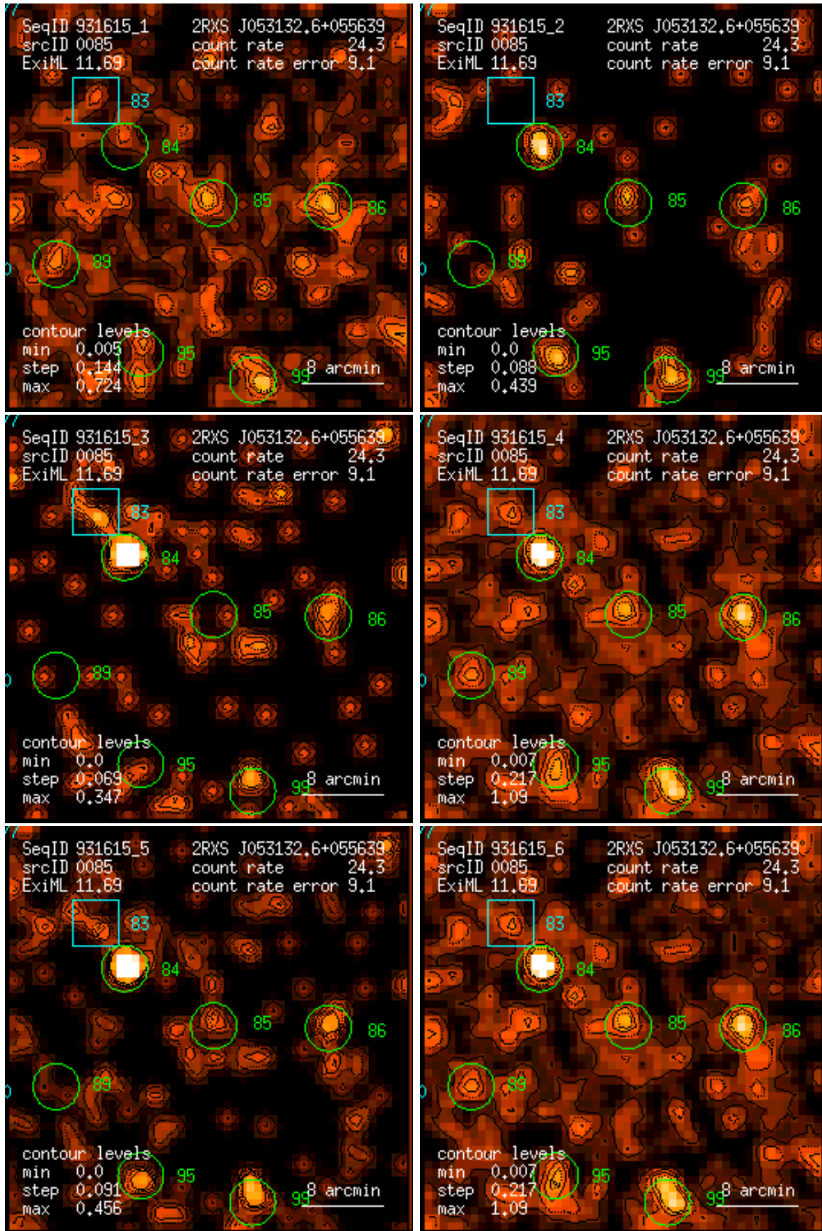
Figure 85: RASS 931615: detection 0085: band rate images, Gaussian filter: (1) PSPC channels 11 – 41, (2) 52 – 90, (3) 91 – 201, (4) 11 – 235, (5) 52 – 201, (6) 11 – 201. Broad band rates in counts/ks. Band rate contour levels in counts/ks/arcmin 2 .
